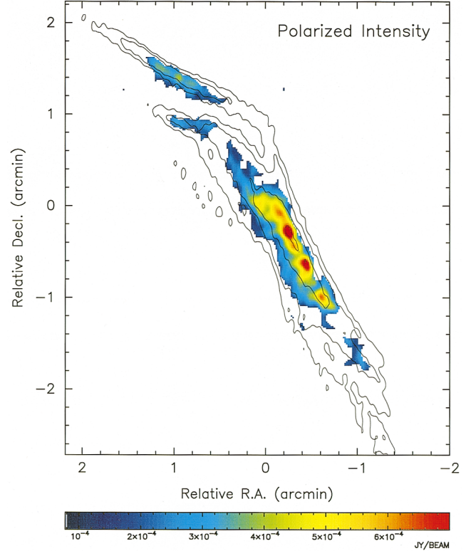
FIG. 2.—Total intensity and polarized emission at 6 cm arising from the Pelican, shown in right ascension and declination units of arcminutes offset from the phase center ( \alpha, \delta_{\text{B1950}} = 17^{\text{h}}37^{\text{m}}48^{\text{s}}.7, -29^\circ38'17''.0 ). The contours show the total intensity with a resolution of 8''.36 \times 3''.54 , P.A. = -1^\circ , and an rms noise level of 20 \mu\text{Jy beam}^{-1} . The contour levels represent 0.1, 0.2, 0.4 , and 0.8 \text{ mJy beam}^{-1} . The polarized emission is shown in false-color scale with a resolution of 9'' \times 5'' , in the range of 150\text{--}700 \mu\text{Jy beam}^{-1} .
