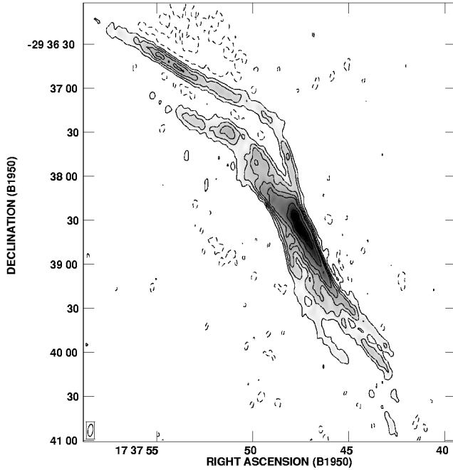
FIG. 1.—The 20 cm continuum image of the Pelican shown in both contours and negative gray scale. The resolution of this image is 8''.43 \times 3''.39 , P.A. = -7^\circ , and it has been corrected for primary-beam attenuation. The rms noise in this image is 55 \mu\text{Jy beam}^{-1} . The contour levels represent -0.2, 0.2, 0.4, 0.6, 0.8, 1, 1.4, 1.8, 2.0 , and 2.2 \text{ mJy beam}^{-1} .
