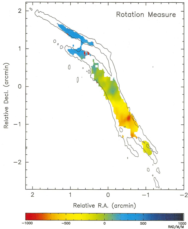
FIG. 3.—The distribution of the RM along the Pelican is shown in false-color scale with units of \text{rad m}^{-2} , superposed with the 0.2 \text{ mJy beam}^{-1} contour of total 20 cm intensity from Fig. 1. The right ascension and declination axes are the same as in Fig. 2.
