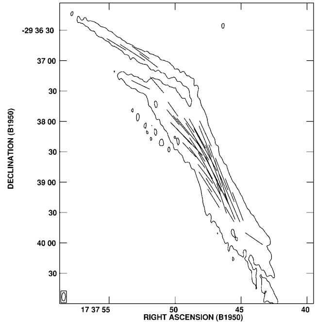
FIG. 4.—The vectors representing the intrinsic orientation of the magnetic field in the Pelican are shown superposed on the 0.2 \text{ mJy beam}^{-1} contour of 6 cm continuum emission from Fig. 2.
