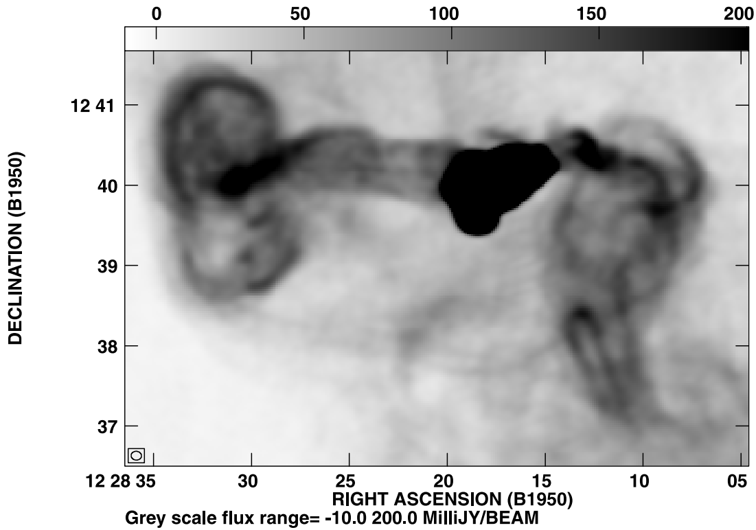
FIG. 2.—90 cm image of central part of Virgo A/M87 radio halo shown in Fig. 1. This display shows the sharp surface brightness drop between the inner radio-lobe structure (which contains the galactic nucleus and the well-known jet; solid black in this figure) and the east and west outflows that emerge from the inner lobes.
