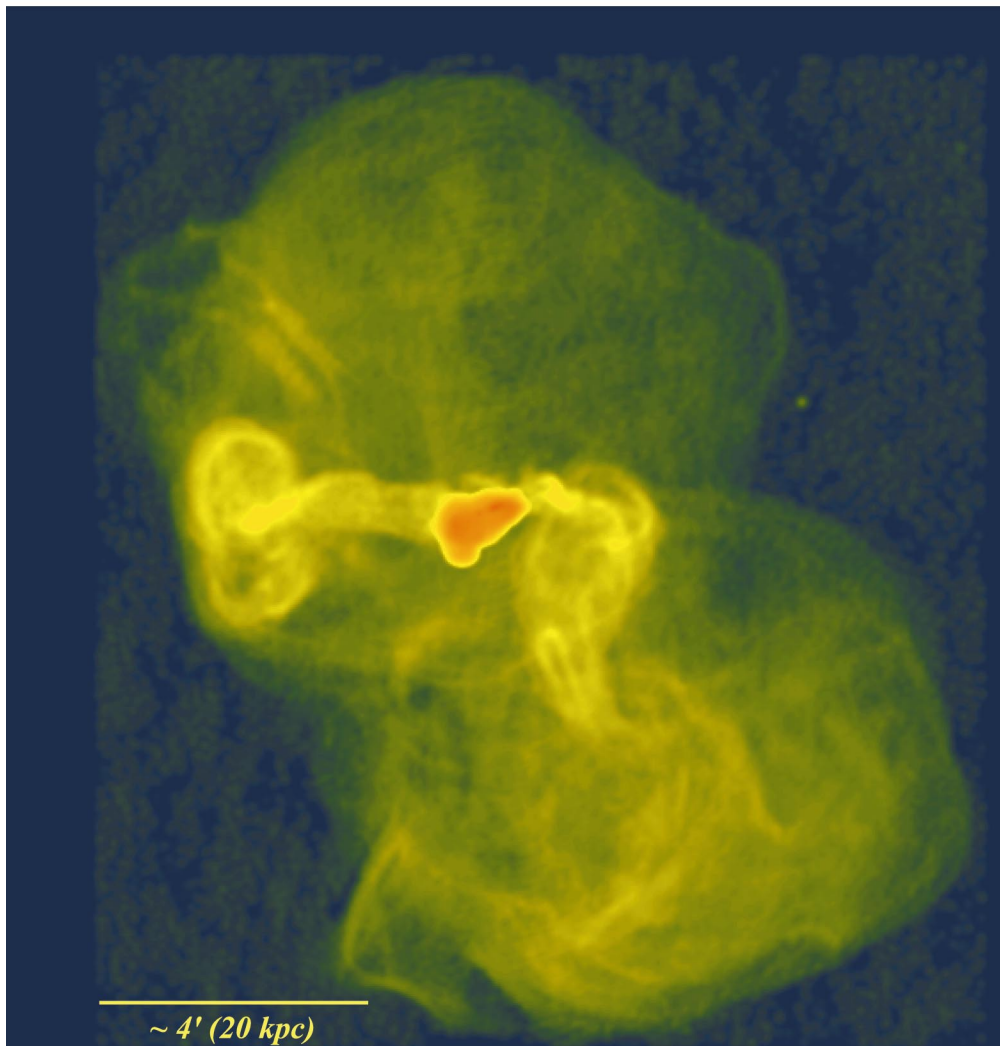
FIG. 1.—90 cm image of M87. The central region containing the jet and inner radio lobes is in the red-orange region near the image center. The convolving beam for this maximum entropy image is 7''.8 \times 6''.2 , P.A. = 86^\circ . One arcsecond corresponds to 85 pc at our assumed distance of 17 Mpc.
