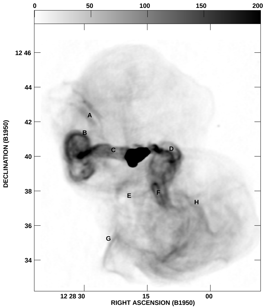
FIG. 3.—Gray-scale image of Virgo A/M87 and the location of minimum-pressure measurements given in Table 1
