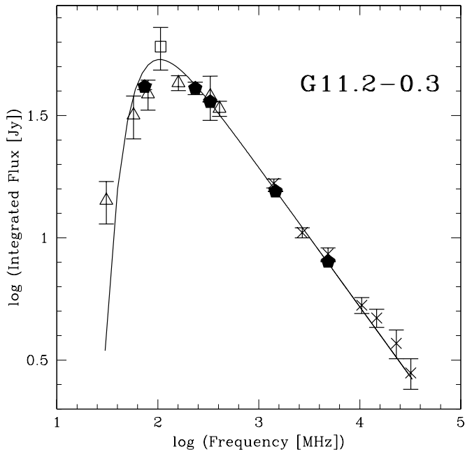
FIG. 2.—Radio continuum spectrum for SNR G11.2–0.3. The best-fit spectral index using eq. (1) is -0.570 \pm 0.002 . The hexagon symbols are from the current work, the triangles are from Kassim (1989b, 1992), the single square is from Kovalenko, Pynzar, & Udaltsov (1994), and the crosses are from Kotthes & Reich (2001). To obtain the spectral index for only the shell of the SNR, 1 Jy has been subtracted from the integrated flux measurements for data with \nu > 200 MHz, assuming that \alpha_P \sim 0.0 .
