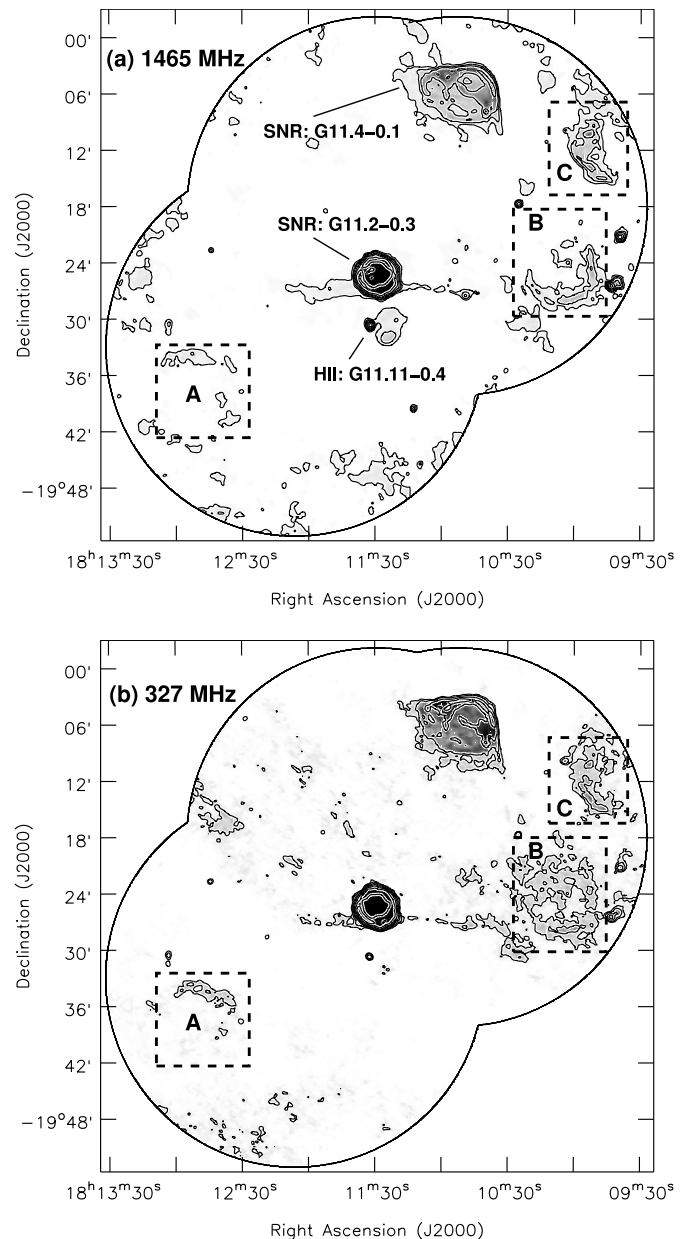
FIG. 1.—(a) VLA 1465 MHz three-pointing mosaic centered on the known SNR G11.2–0.3 with 25'' resolution. The contour levels are 4, 10, 20, 50, 100, 200, and 400 mJy beam -1 . The rms noise of this image is \sim 1 mJy beam -1 but varies somewhat as a function of position as a result of the mosaicking procedure. The sources identified with the dotted boxes and labeled A, B, and C are the three new SNR candidates. (b) VLA image at 330 MHz centered on SNR G11.2–0.3 with 25'' resolution. The contour levels are 10, 20, 50, 100, 200, 400, and 700 mJy beam -1 . The rms noise of this image is \sim 3 mJy beam -1 . The region outside of the 1465 MHz mosaic has also been blanked on the 330 MHz image for ease of comparison.
