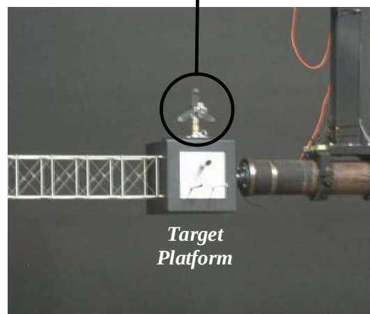
Figure 9. Pursuer and target platform hardware.
