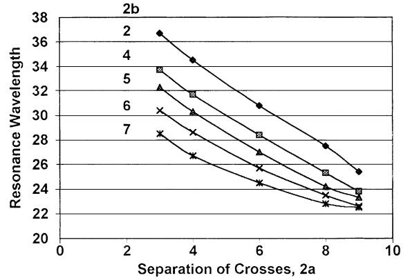
Fig. 2. Micro-Stripes calculations of the resonance wavelength of free standing inductive cross shaped metal mesh of thickness 0.2 \mu\text{m} and using a surface impedance Z = 1.635 \Omega\text{cm} . The dependence on the separation of the crosses and the width of the cross arms is shown for the range of a/g = 0.075, 0.1, 0.15, 0.2, 0.225 and b/g = 0.05, 0.1, 0.125, 0.15 and 0.175 .
