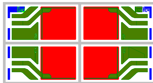
Figure 14: Cat's eye array photolithography mask
