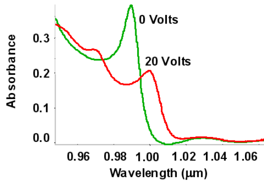
Figure 4: The band-edge optical absorption of a MQW for 0 and 20 V reverse bias
