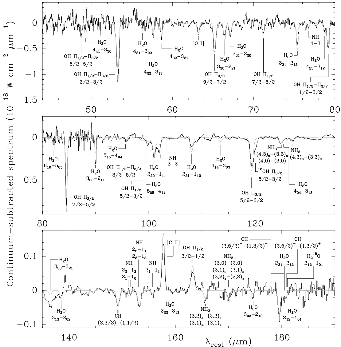
FIG. 7.—Continuum-subtracted spectrum of Arp 220, compared with the result of the model ( in gray ). The line features that contribute more to the model are identified (see text).
