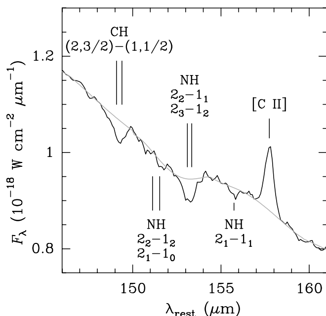
FIG. 3.—Line assignments in the vicinity of the 153.2 \mu\text{m} feature. The gray line shows the adopted continuum level.
