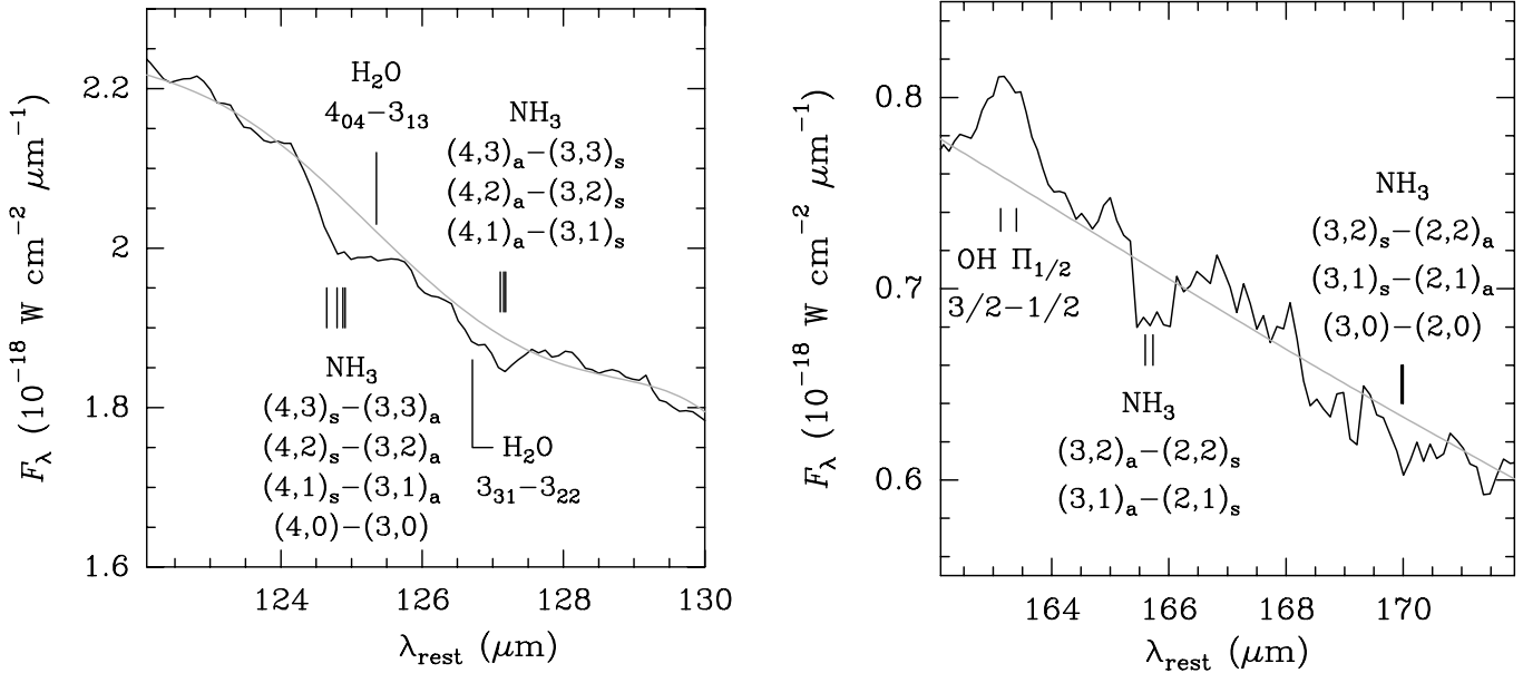
FIG. 4.—NH 3 lines around 125, 127, 166, and 170 \mu\text{m} . The gray line shows the adopted continuum level. The 125 and 127 \mu\text{m} features could be partially contaminated by the labeled H 2 O lines.
