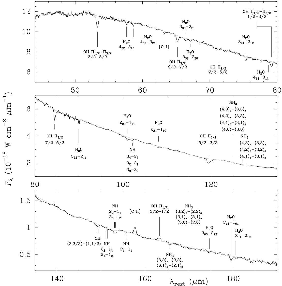
FIG. 1.—ISO LWS spectrum of Arp 220, where the most prominent line features are identified (see text). The gray line shows the adopted baseline (continuum level). Wavelengths in this and following figures are rest wavelengths.
