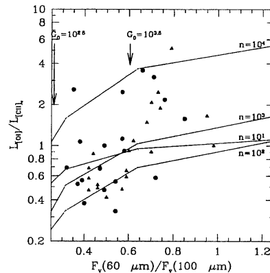
Figure 5. As in Figure 4, but here a correction is made for [C\ II] arising from the diffuse ionized medium, based on [N\ II]122 observations. The triangles denote galaxies where [N\ II] 2- \sigma upper limits were used. From Malhotra et al. (2000b).
