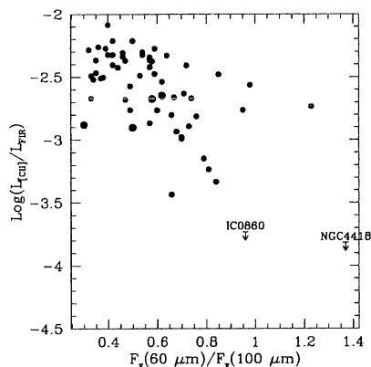
Figure 2. The [C II]158/FIR flux ratio versus F_{60}/F_{100} from IRAS. Early-type galaxies are denoted by bullseye symbols. From Malhotra et al. (2000a).
