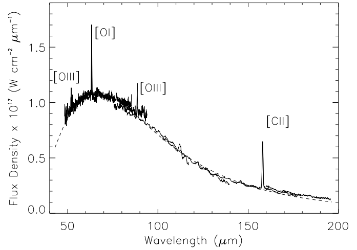
Fig. 2. LWS spectrum of the central region of the dust lane (dashed line is the blackbody fit)
