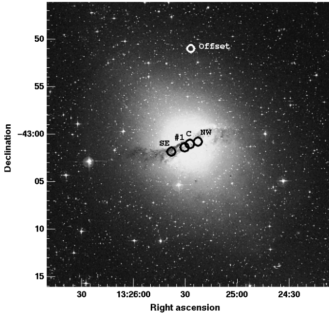
Fig. 1. Cen A digital sky survey image overlaid with the LWS beam positions
