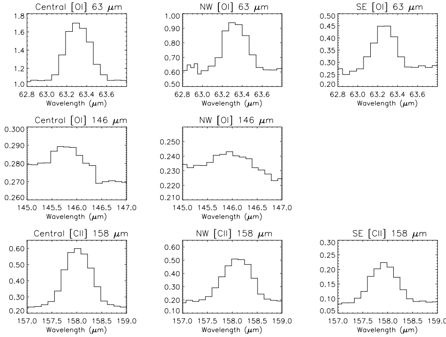
Fig. 3. PDR Lines (Flux Density \times 10^{17} W cm ^{-2} \mu m ^{-1} ). Note the [C II] lines are the total observed flux density i.e. PDR + CNM + WIM
