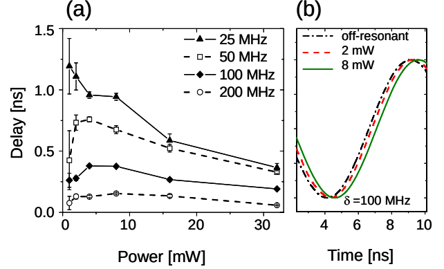
FIG. 4. (a) Power dependence of the time delay at various modulation frequencies. (b) Off-resonant modulation trace and resonant modulation traces at powers of 2 and 8 mW ( \delta = 100 \text{ MHz} ) demonstrating controllable delay.
