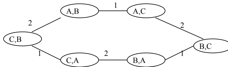
Figure 2: Kripke model for the card game.
