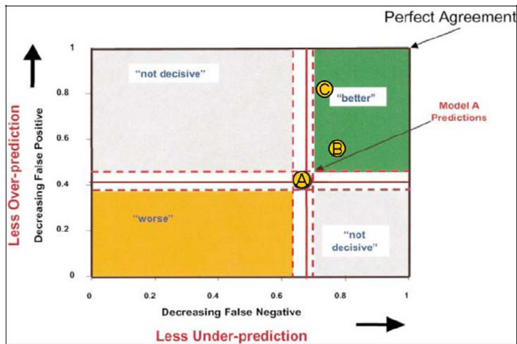
Figure 10. Regions of predictability in MOE, model comparison
