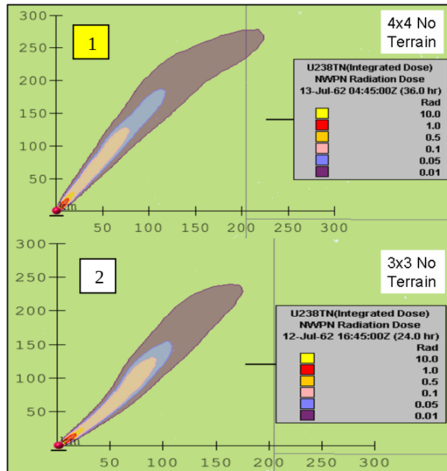
Figure 74. Johnnie Boy, NWP terrain only
