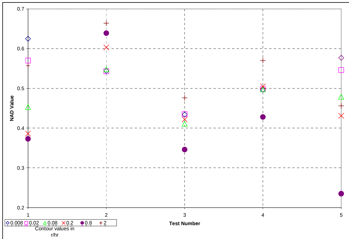
Figure 35. Comparison of ESS NAD values by test, lower value is better
