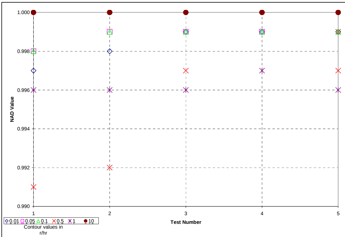
Figure 76. Comparison of Johnie Boy NAD values, lower value is better
