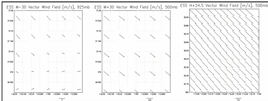
Figure 31. ESS vector wind fields
