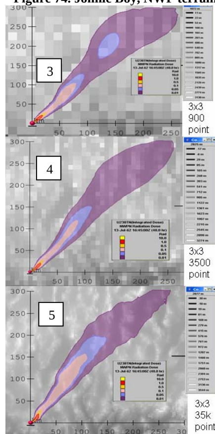
Figure 75. Johnnie Boy, various terrain resolutions
