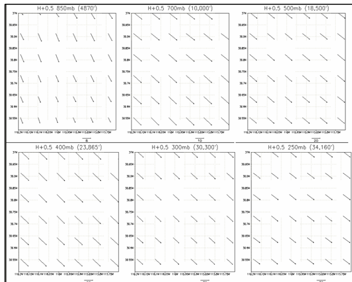
Figure 37. ESS expanded wind field
