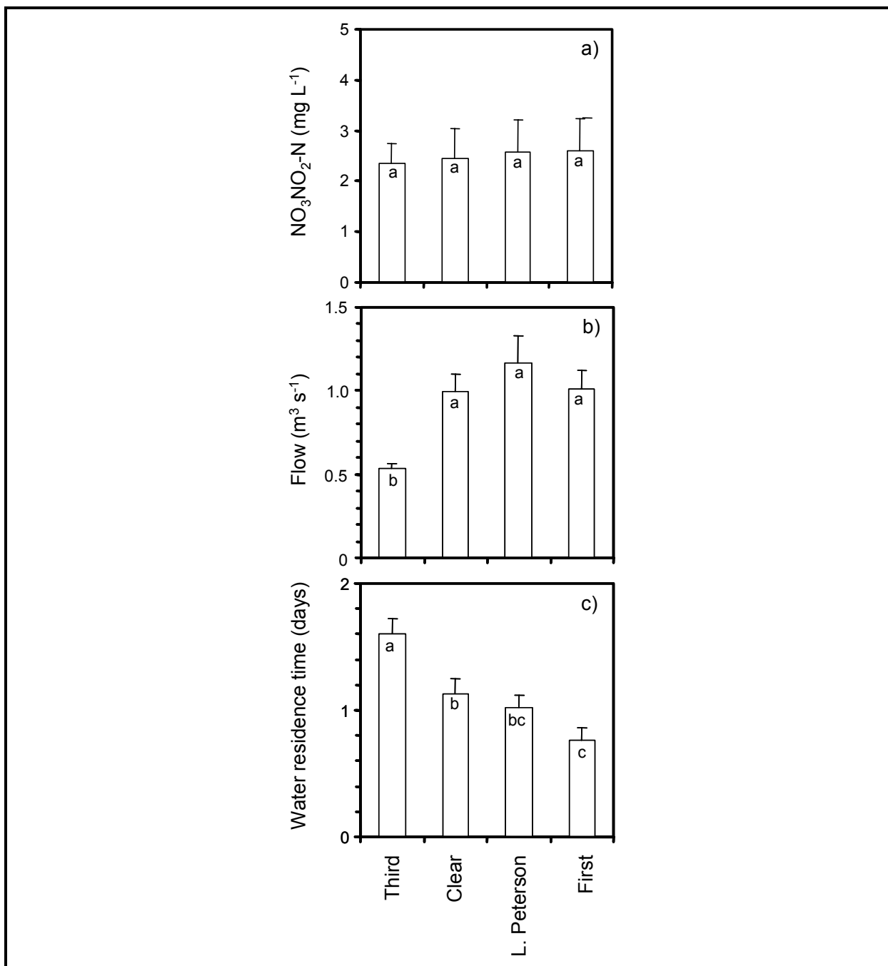
Figure 3. Mean summer (a) nitrate-nitrite-N ( \text{NO}_3\text{NO}_2\text{-N} ) concentration, (b), culvert flow, and (c) water residence time for various backwater lakes. Vertical lines represent 1 standard error. Letters represent significant differences in the mean at the 5-percent level or less (ANOVA; Statistical Analysis System (SAS) 1994)
