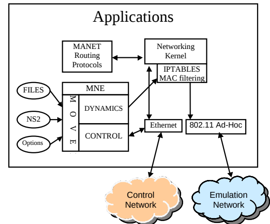
Figure 2 — MNE components
