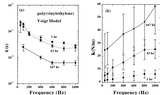
Fig. 4. Voigt model analysis of (a) the response time \tau and (b) stiffness \kappa of the contact showing changes as a function of sample age for PVE.
