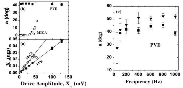
FIG. 2. Shear response (a) amplitude X_t and (b) phase a as a function of drive amplitude X_o for mica and PVE; F_N = 2 \text{ nN} . (c) Frequency dependence of phase lag \alpha for PVE measured at constant load ( \blacksquare 's) and at maximum load during a force-distance curve measurement ( \blacktriangledown 's) such as that shown in Fig. 3.
