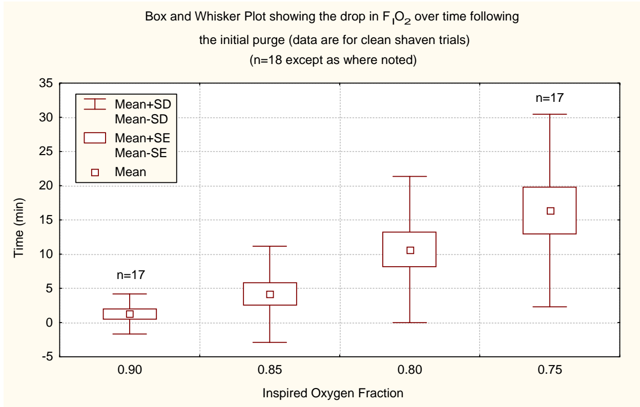
Figure 1: A box and whisker plot showing the average time taken for the concentration of oxygen within the original MBS 2000 closed circuit breathing loop to drop to various F_{iO_2} levels following the initial purge. Data are based on n=18 except as where noted. From Fothergill (2005a).
