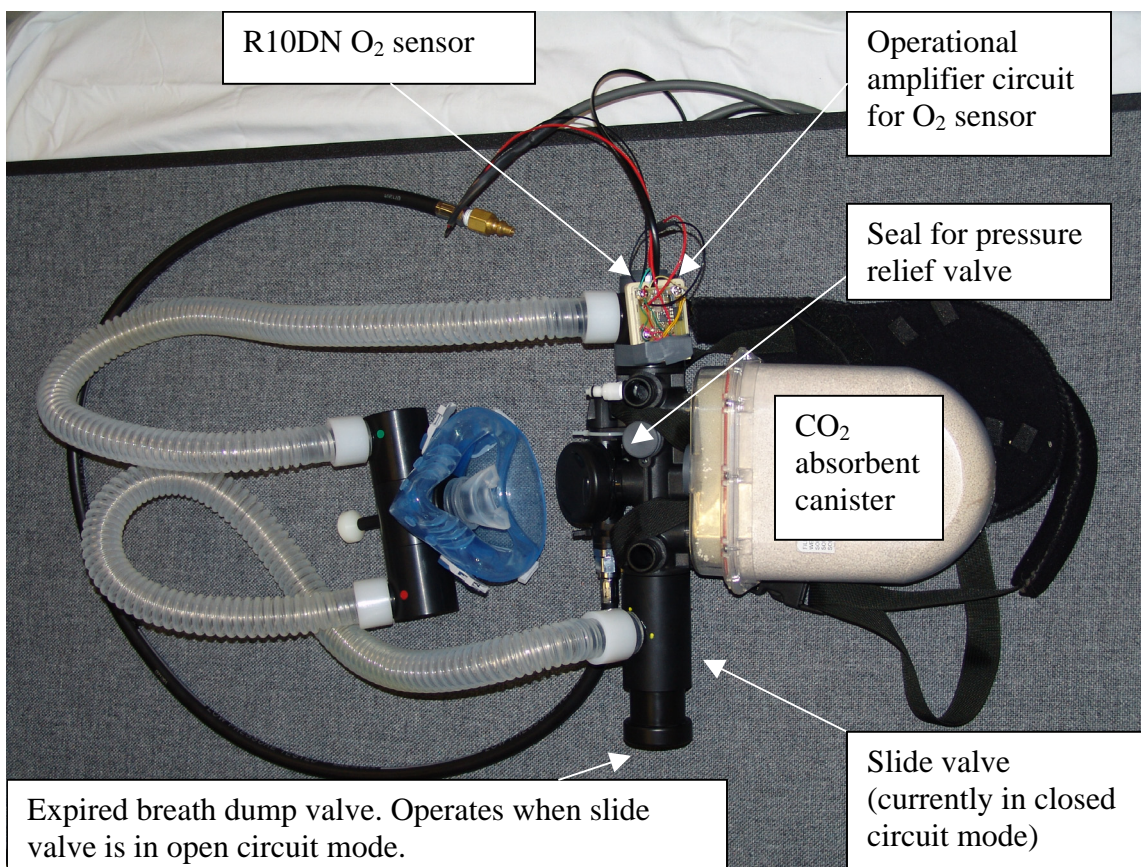
Figure 3: A photo of the modified MBS 2000 without the breathing bags showing the new slide valve attached to the main body on the expired side of the circuit. When the slide valve is placed in the open circuit position (slide valve pushed out to the full lateral position [i.e. downwards toward the expired end cap in the above picture]) expired breath is directed out of the closed circuit through a one way valve in the end cap of the slide valve. The R10-DN O 2 sensor together with its prototype operational amplifier is shown on the inspired side of the MBS 2000 main body.
