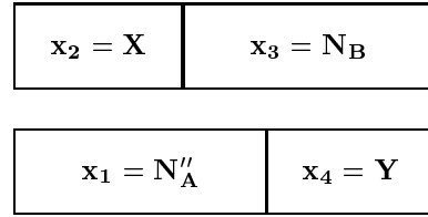
Figure 1. Messages obeying \mathbf{C}_1 constraints
