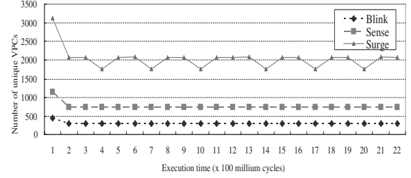
Figure 11. Number of unique VPCs executed in three applications
