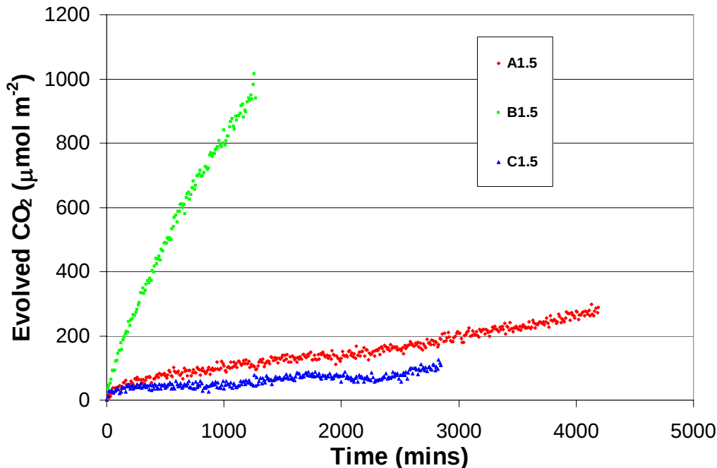
Figure 6: CO 2 vs time profile for X1.5 samples irradiated with UVA containing no pigment (blue), a stable grade A pigment (red) and an unstable anatase pigment (green).
