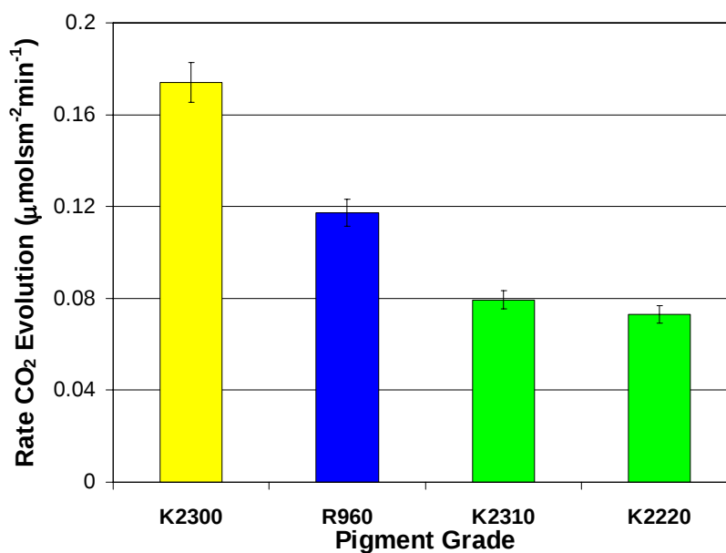
Figure 4: \text{CO}_2 evolution rates as a function of pigment type. NB K2220 and K2310 are grade A pigments and K2300 is a grade B material. R960 is the rutile \text{TiO}_2 used in the USAF polyurethane coatings.
