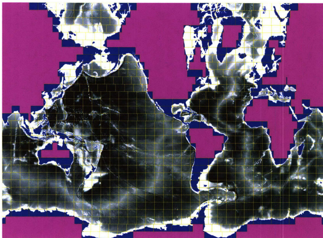
Figure 2. Current tiling for the 1/12^\circ global domain with equal-sized tiles that (a) allows rows to be offset from each other if this gives fewer tiles over the ocean and (b) allows two tiles to be merged into one larger tile if less than 50 percent of their combined area is ocean. The Mediterranean region especially illustrates both these optimizations; out of the original 1152 (36 by 32) approximately equal-sized tiles, 371 tiles are entirely land and are discarded, leaving 781. The Arctic "wraps" between the left and right halves of the top edge.
