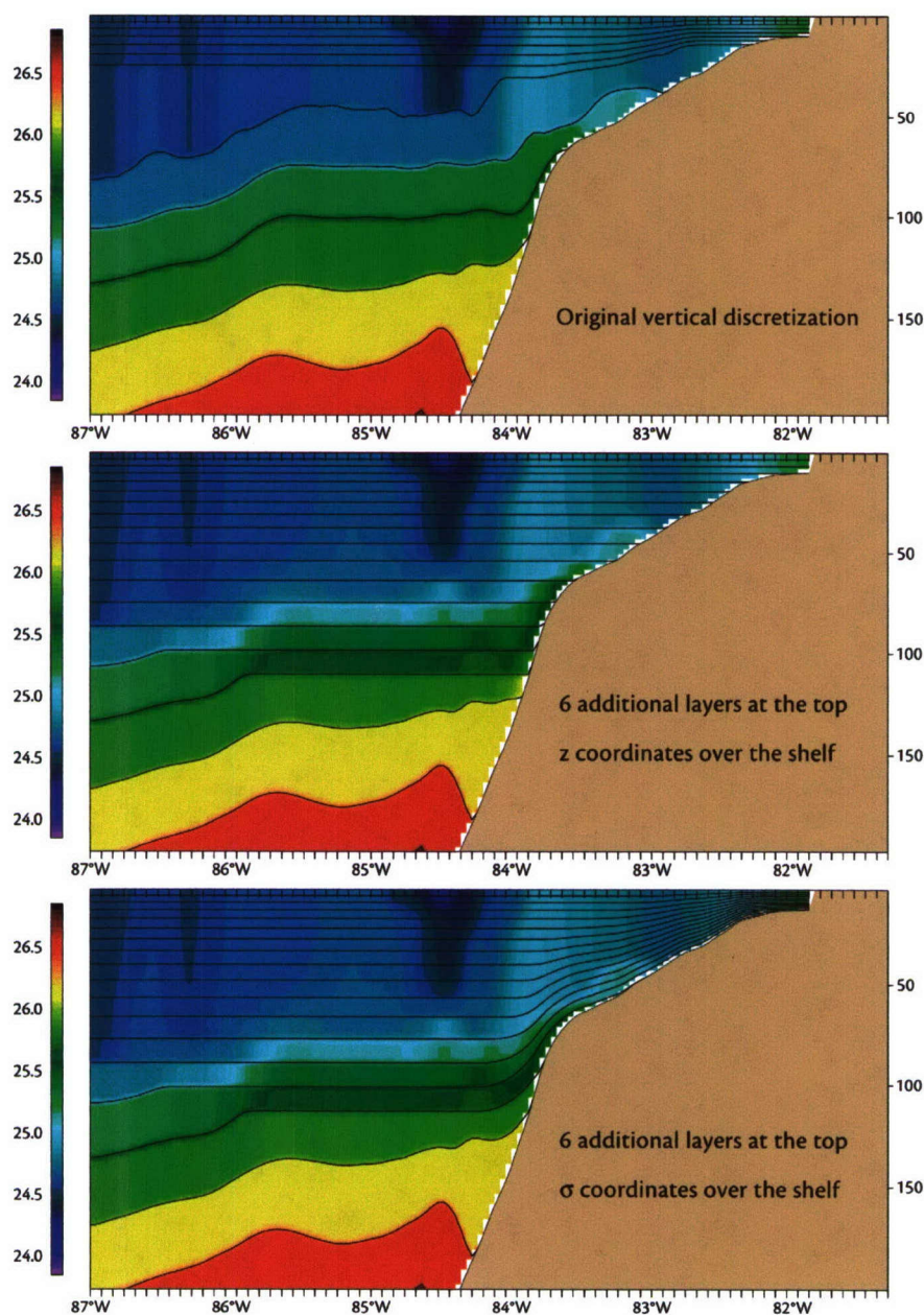
Figure 1. Cross sections of layer density and model interfaces across the West Florida Shelf in a 1/25^\circ West Florida Shelf subdomain covering the Gulf of Mexico east of 87^\circ\text{W} and north of 23^\circ\text{N} and embedded in a 1/12^\circ Atlantic basin HYCOM simulation (Halliwell et al., in preparation). This figure illustrates the transition among pressure, terrain-following, and isopycnal coordinates in 1/25^\circ West Florida Shelf simulations nested within a 1/12^\circ North Atlantic configuration, and it demonstrates the flexibility with which vertical coordinates can be chosen and the capability of adding additional vertical resolution.
