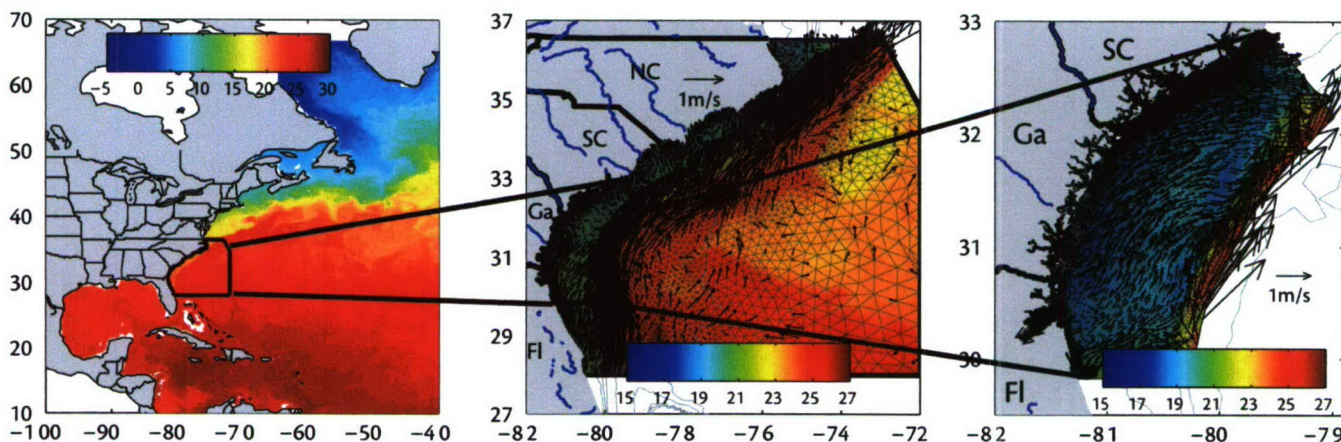
Figure 4. (Left) 1/12° North Atlantic HYCOM-GODAE sea surface temperature (SST) nowcast for November 28, 2005. The three-dimensional solution for this date is used to initialize the University of North Carolina-South Atlantic Bight (UNC-SAB) finite element modeling system (middle, every 5 th model vector). The surface temperature and velocity are shown, after addition of the regional tides and atmospheric fluxes. The limited-area finite element implementation (right, every 3 rd model vector) includes the estuary and tidal inlets along the Georgia/South Carolina coast and extends to the shelf-break. This snapshot also shows surface temperature and velocity and is for three days after initialization. The color scales between the HYCOM and nested plots are not the same.
