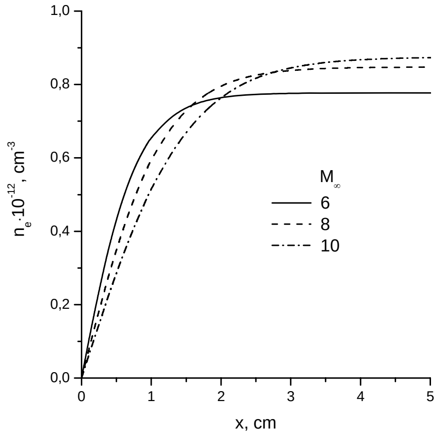
Fig.3. Spatial dependencies of electron concentration in FS region at q_{ion}=1\text{W}/\text{cm}^3 , q_\infty=75 \text{ kPa} .
