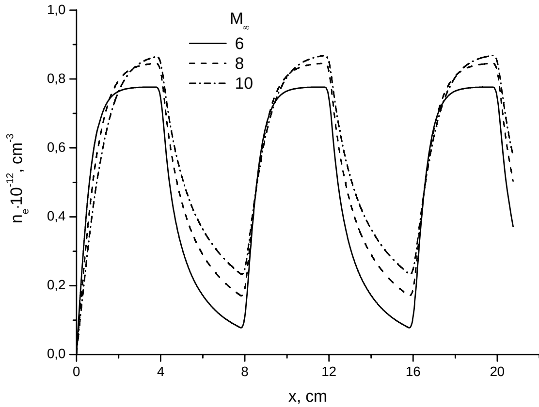
Fig.6. Electron concentration in FS region for periodically spaced e-beams with f(x) shown in fig.5 at q_{ion}=1\text{W}/\text{cm}^3 , q_\infty=75 kPa, \Delta x=4 cm, \delta x=4 cm.
