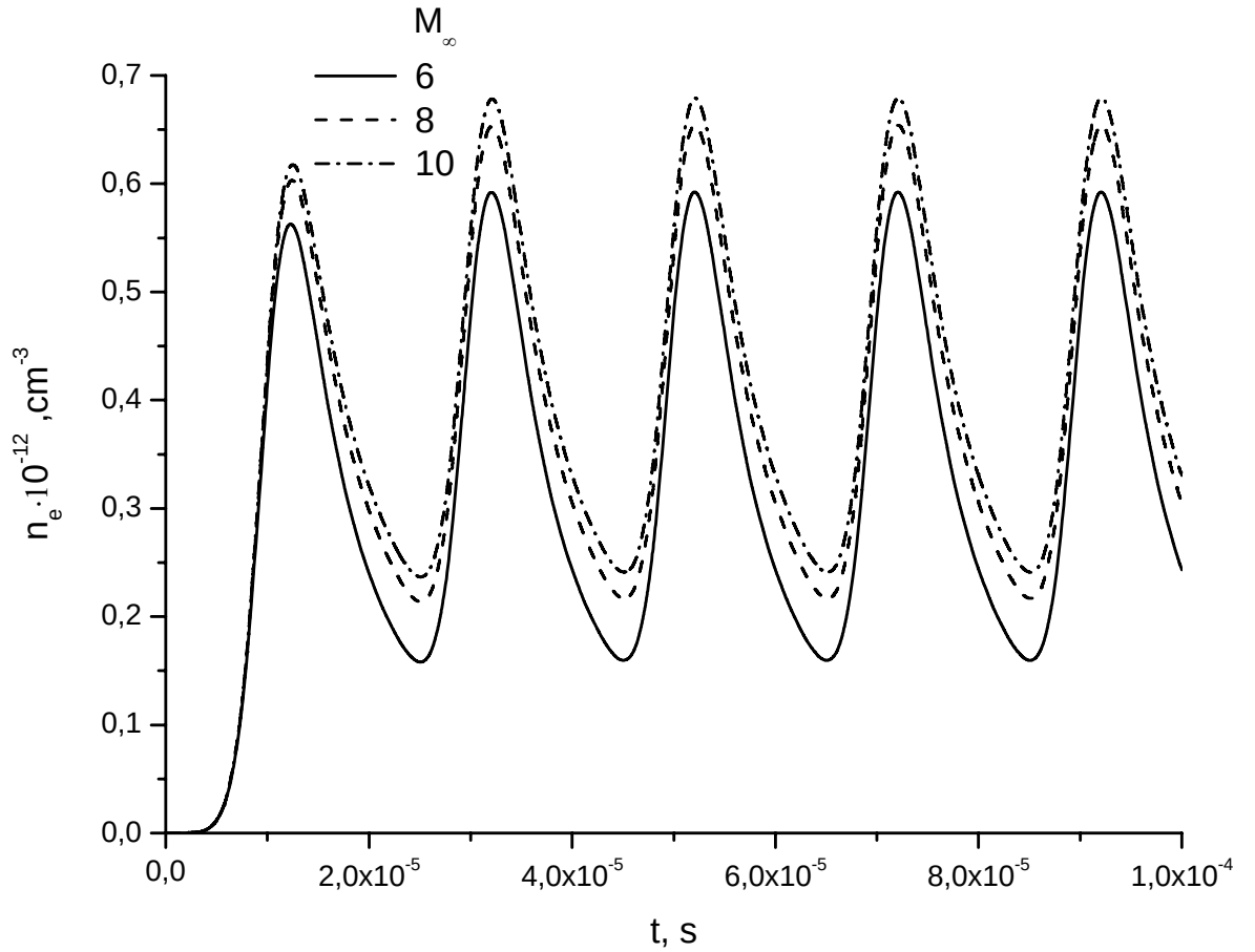
Fig.10 Time-dependent electron concentration in uniform plasma sustained by pulse-periodic e-beam with T=2 \cdot 10^{-5}\text{ s} in FS region at q_{ion}=1\text{W}/\text{cm}^3 , q_{\infty}=75\text{ kPa} .
