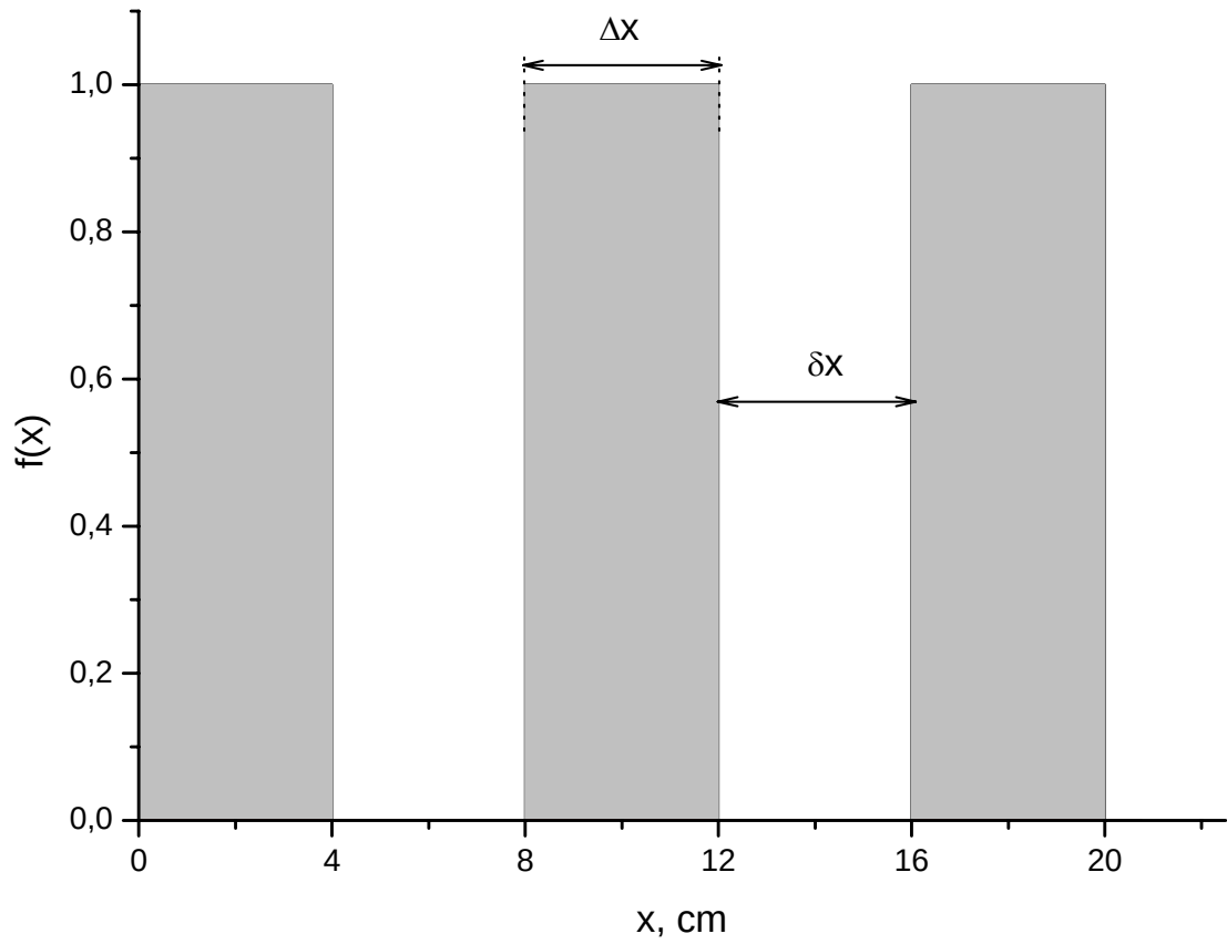
Fig.5. Function f(x) for periodically spaced e-beams in form of a slab with \Delta x=4 cm, \delta x=4 cm.
