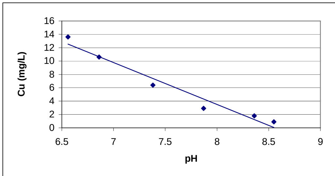
Figure 10. Soluble Copper (0.2 \mu\text{m} filter) vs pH
