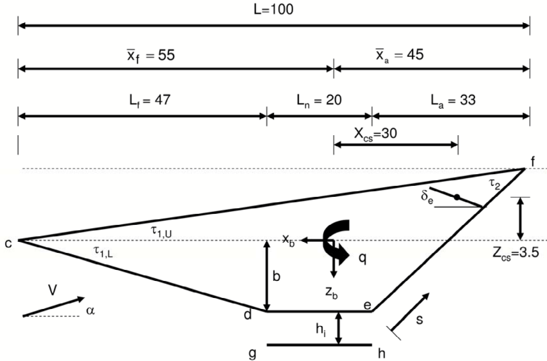
Figure 1. Hypersonic Vehicle.
