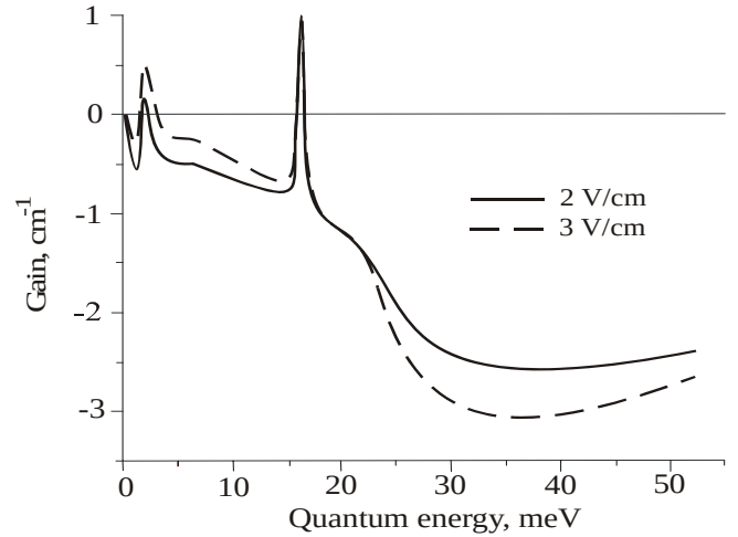
Fig. 30. Optical gain spectrum in uniaxially strained p-Ge for 4 kbar pressure along [100] direction.
