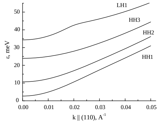
Fig. 46. Energy dispersion of valence band of Si/Si 0.85 Ge 0.15 /Si QW structure.
