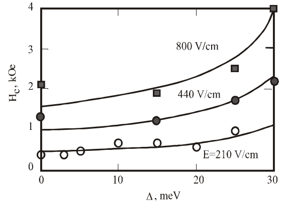
Fig. 34, b. Critical magnetic field H_c vs valence band splitting \Delta . Lines show the calculated H_c(\Delta) dependence.
