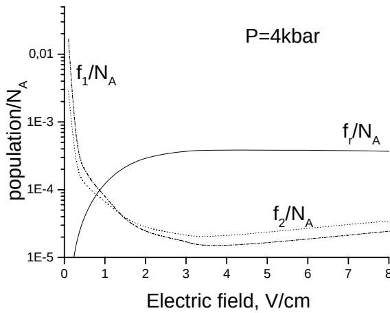
Fig. 29. Electric field dependence of acceptor-state population.
