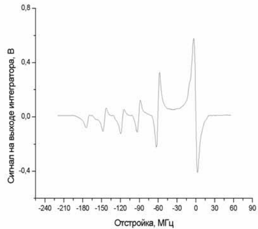
Fig.22. Discrimination curve for resonances at the 5S_{1/2} (F = 3) \rightarrow P_{3/2} (F = 2, 3, 4) transition obtained by modulating the longitudinal magnetic field in the reference cell with ^{85}\text{Rb} and detecting synchronously the difference absorption signal of two probe beams. The saturating beam intensity is 0.1 \text{ mW cm}^{-2} and the recording time is 120s.
