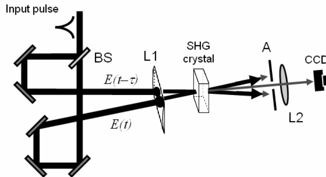
Fig. 3.1.2.2 Scheme of the single-short autocorrelator processing. BS – beam splitter, L1 – cylinder lens, A – aperture, CCD – CCD-camera, L2 – lens for imaging on the CCD-camera.
