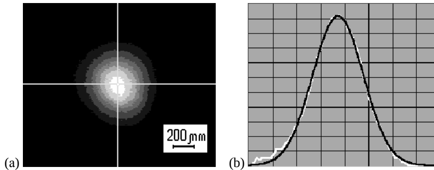
Fig. 3.1.2.5 Beam image at the lens focus with F/D=8 (a) and its X-axis profile & Gaussian fit (b). Magnification factor M=47 , \lambda=1240 nm.
