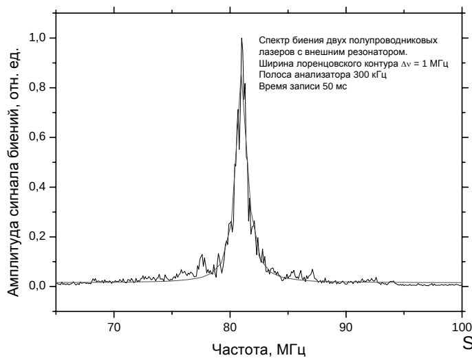
Fig. 15 Master lasers beat note spectrum. The spectrum width is lower than 1.5 MHz.
