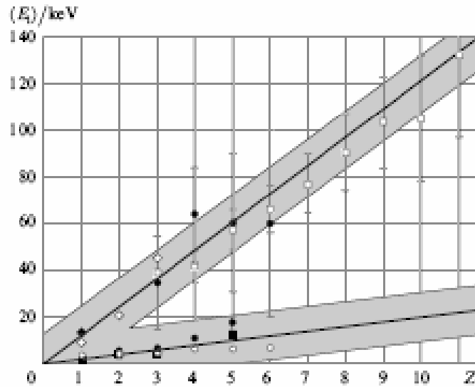
Figure 3.3.5.6. Average ion energies \{E_i\} as functions of Z for an unpurified target ( \diamond — protons, \bullet — C, \square — O, \blacksquare — Si) and a target cleaning with delays At = 100 us ( d — high-energy Si component, o — low-energy Si component) and At = 400 ns ( o — Si).
