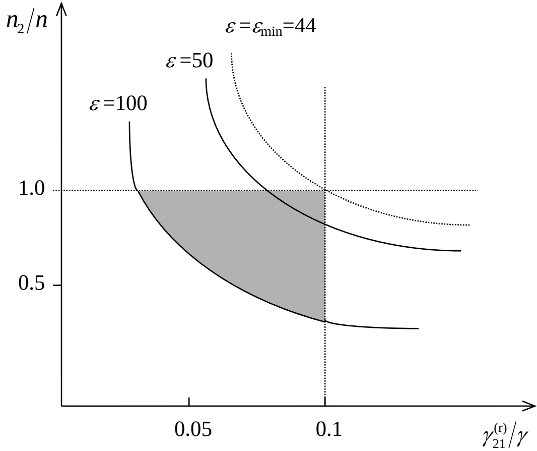
Fig. 3. Relative concentration of excited nuclei, n_2/n , against the linewidth ratio \gamma_{21}^{(r)}/\gamma with \varepsilon = \lambda_0^2 nL taken as a parameter of a family of curves (the internal electron conversion coefficient is assumed to be \alpha = 10 ).
