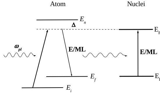
Fig. 4.1.3. Scheme of the nuclear excitation by photons via an atomic shell.
