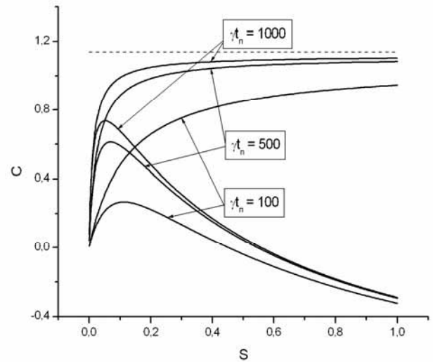
Fig. 26. Theoretical dependences of the nonlinear contrast c_h ( (A_h - A_n)_{\text{opt}} / A_n ) at the cyclic transitions from the F \sim 2 level of the ground state of ^{87}\text{Rb} on the saturation parameter S . The upper curve in each pair of curves for the same value of \gamma t_n corresponds to the scheme with the screening of the central part of the saturating beam. The horizontal dashed curve is the ultimate contrast (114 %) discussed in the text.
