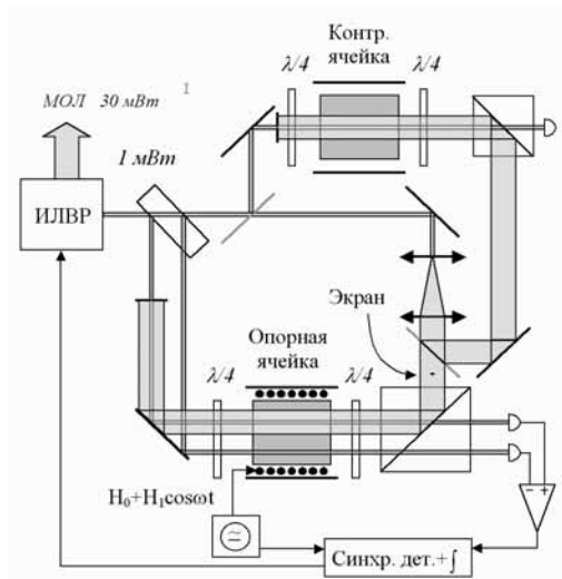
Fig. 21. Scheme for frequency stabilisation of an diode laser with an external resonator (DLER) by the sub-Doppler absorption resonance in an atomic cell.
