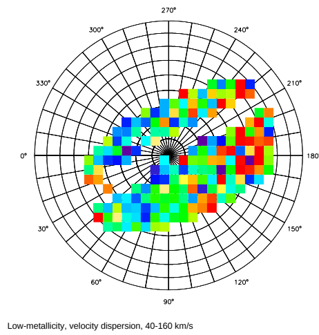
Fig. 6. Analogous to Fig. 5, except that the velocity dispersion is shown (color-coded from 40 km/s to 160 km/s).
