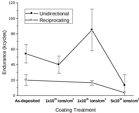
Figure 5. Unidirectional (POD) and reciprocating sliding endurance for as-deposited and ion irradiated IBA \text{MoS}_2 coatings.
