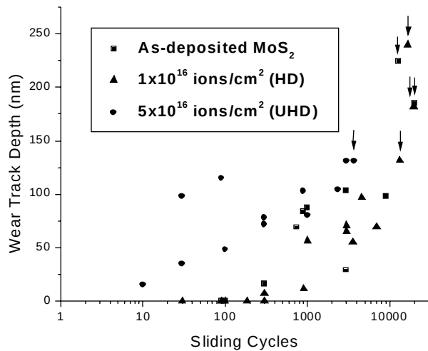
Figure 7. Wear track depths measured by interference microscopy for as-deposited and ion irradiated IBAD MoS 2 coatings. Data points with arrows indicate failure.
