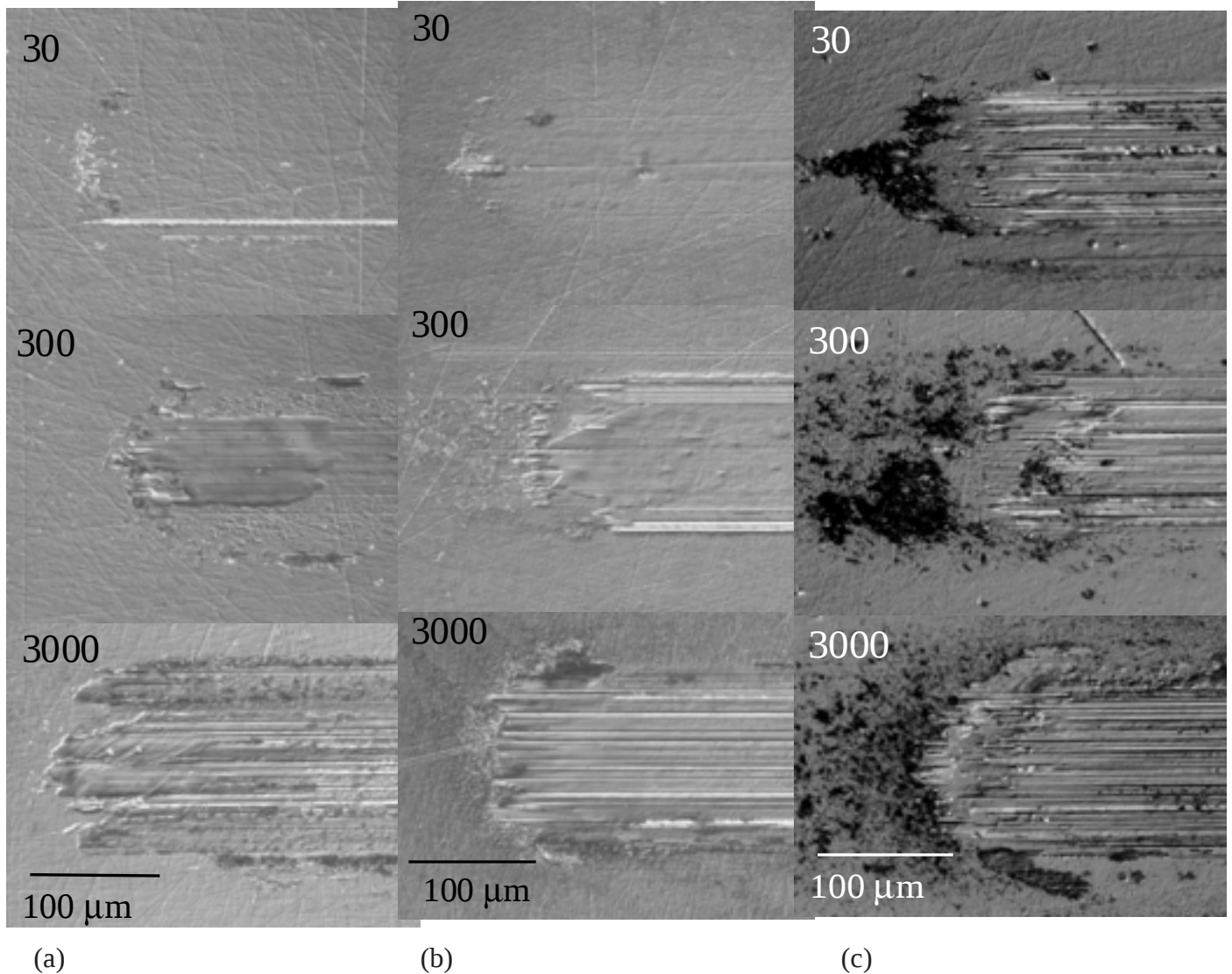
Figure 10. Debris deposited at wear track ends at 30, 300 and 3000 sliding cycles for (a) as-deposited, (b) 1 \times 10^{16} ions/cm 2 (HD) and (c) 5 \times 10^{16} ions/cm 2 (UHD) MoS 2 coatings.
