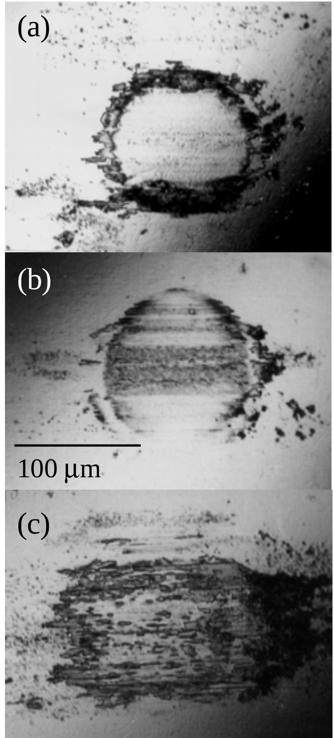
Figure 8. Optical micrographs of ball transfer films after 90 cycles of reciprocating sliding for (a) as-deposited, (b) 1 \times 10^{16} ions/cm 2 (HD) and (c) 5 \times 10^{16} ions/cm 2 (UHD) MoS 2 coatings.
