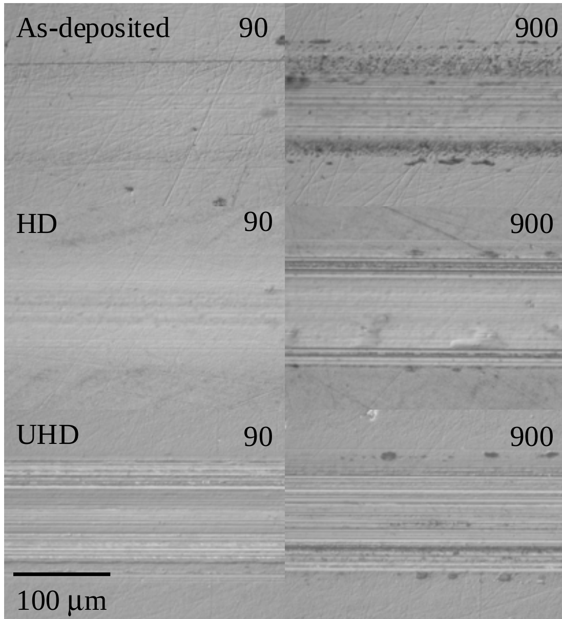
Figure 9. Wear tracks on flats corresponding to ball transfer films shown in Fig. 8 at 90 cycles and at 900 cycles.
