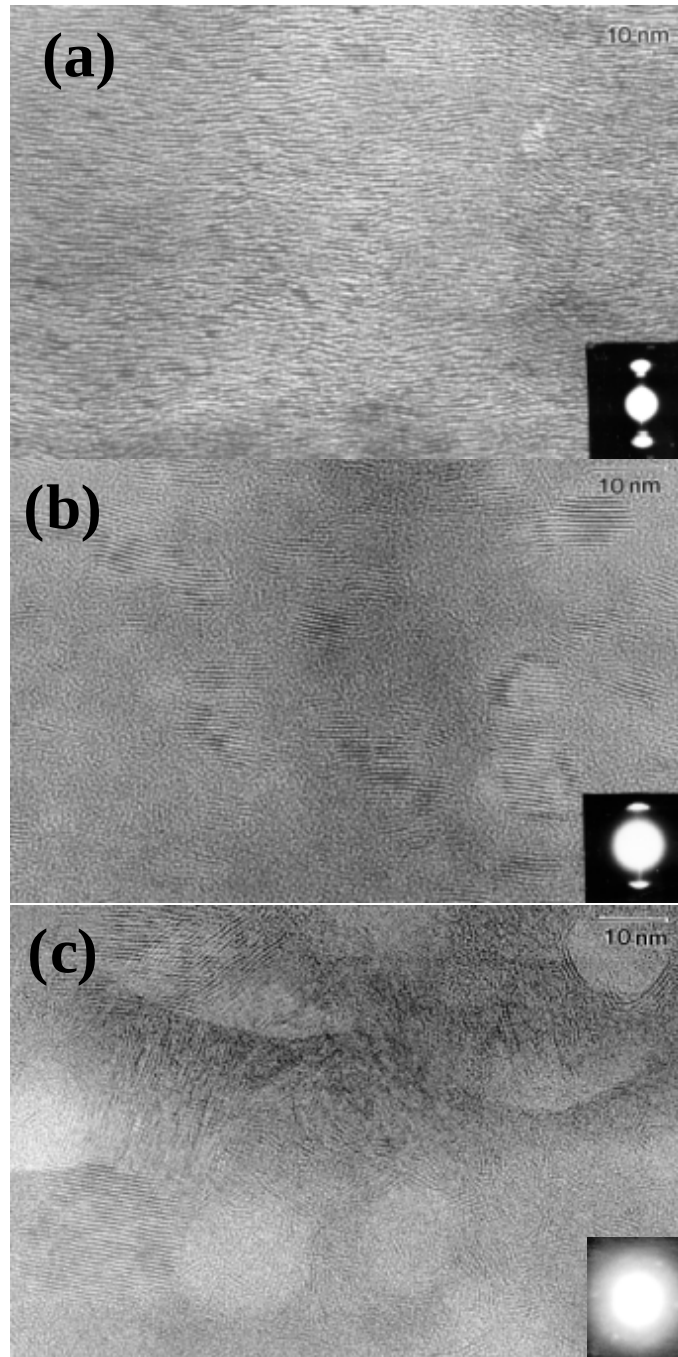
Figure 4. Cross-section TEM images from IBAF \text{MoS}_2 coatings (a) as-deposited, and after irradiation with 180 keV \text{Ar}^{++} ions to (b) 1 \times 10^{15} ions/cm 2 (LD) and (c) 5 \times 10^{16} ions/cm 2 (UHD). Fringes running left to right correspond to \text{MoS}_2 basal planes (S-Mo-S).
