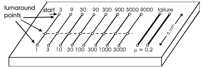
Figure 2. Schematic diagram of reciprocating sliding 'stripe' tests. Arrow marked "start" indicates test starting location, turnaround points are indicated by open circles, and sliding cycles for the track segments are numbered.
