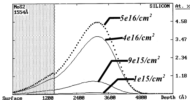
Figure 1. 360 keV Ar + implantation profiles of MoS 2 coated Si at the four doses indicated. Computations assumed atomic densities of 4.8 g/cm 3 for MoS 2 and 2.3 g/cm 3 for Si and pre-irradiation coating thickness of 185 nm. Final thickness (shown) includes sputtering loss.
