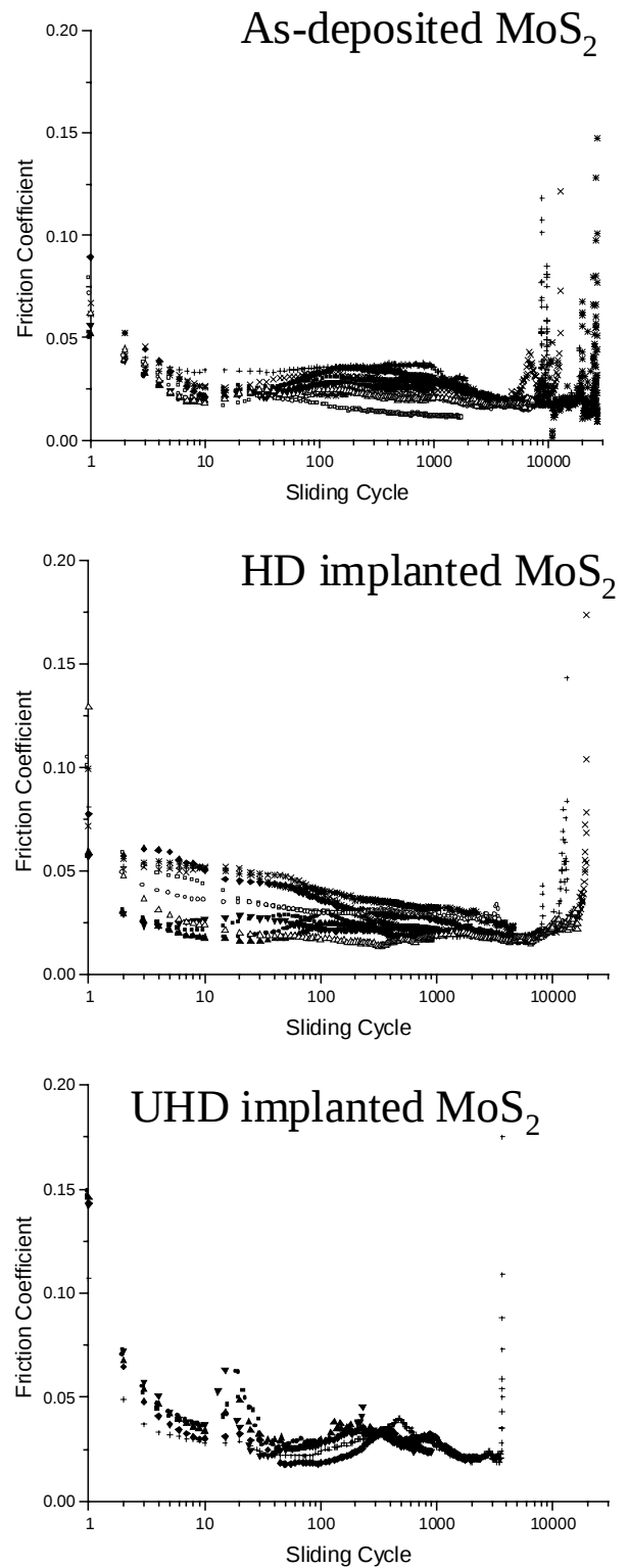
Figure 6. Friction coefficient evolution for reciprocating sliding in dry air against (a) as-deposited, (b) 1 \times 10^{16} ions/cm 2 (HD) and (c) 5 \times 10^{16} ions/cm 2 (UHD) \text{MoS}_2 coatings.
