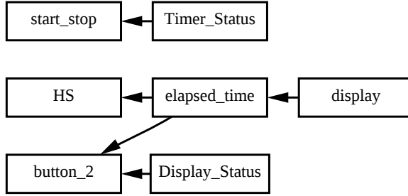
Fig. 1. The dependency graph of module stopwatch.
