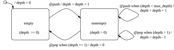
Fig. 6. Visual representation of safestack .
