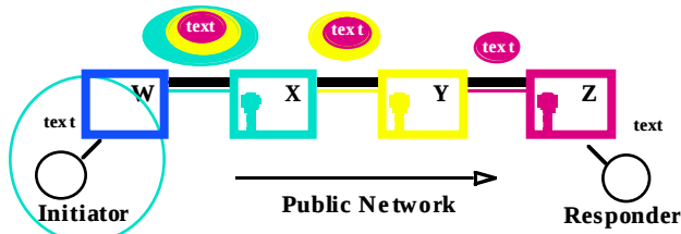
Figure 6: Moving Data Forward
