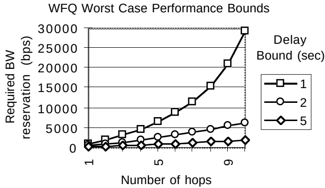
Figure 6: WFQ required bandwidth for latency bound
