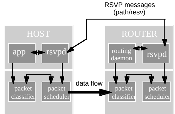
Figure 4: RSVP Host - Router Interaction
