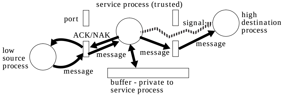
Figure 2. Basic write-up service
