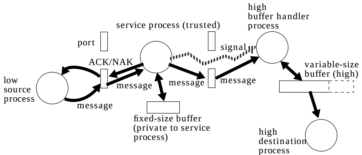
Figure 4. Improved write-up service with variable-size buffer
