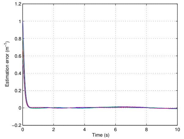
Figure 4: Simulation case 3: Depth estimation error with noise of variance 0.0001 and filtering.
