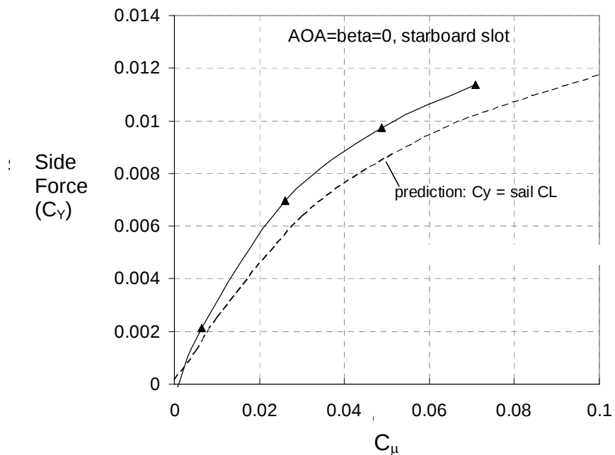
Figure A-32: Test data from figure A-30 with superposition of pretest expected results, under the assumption of no contributions from the body.
