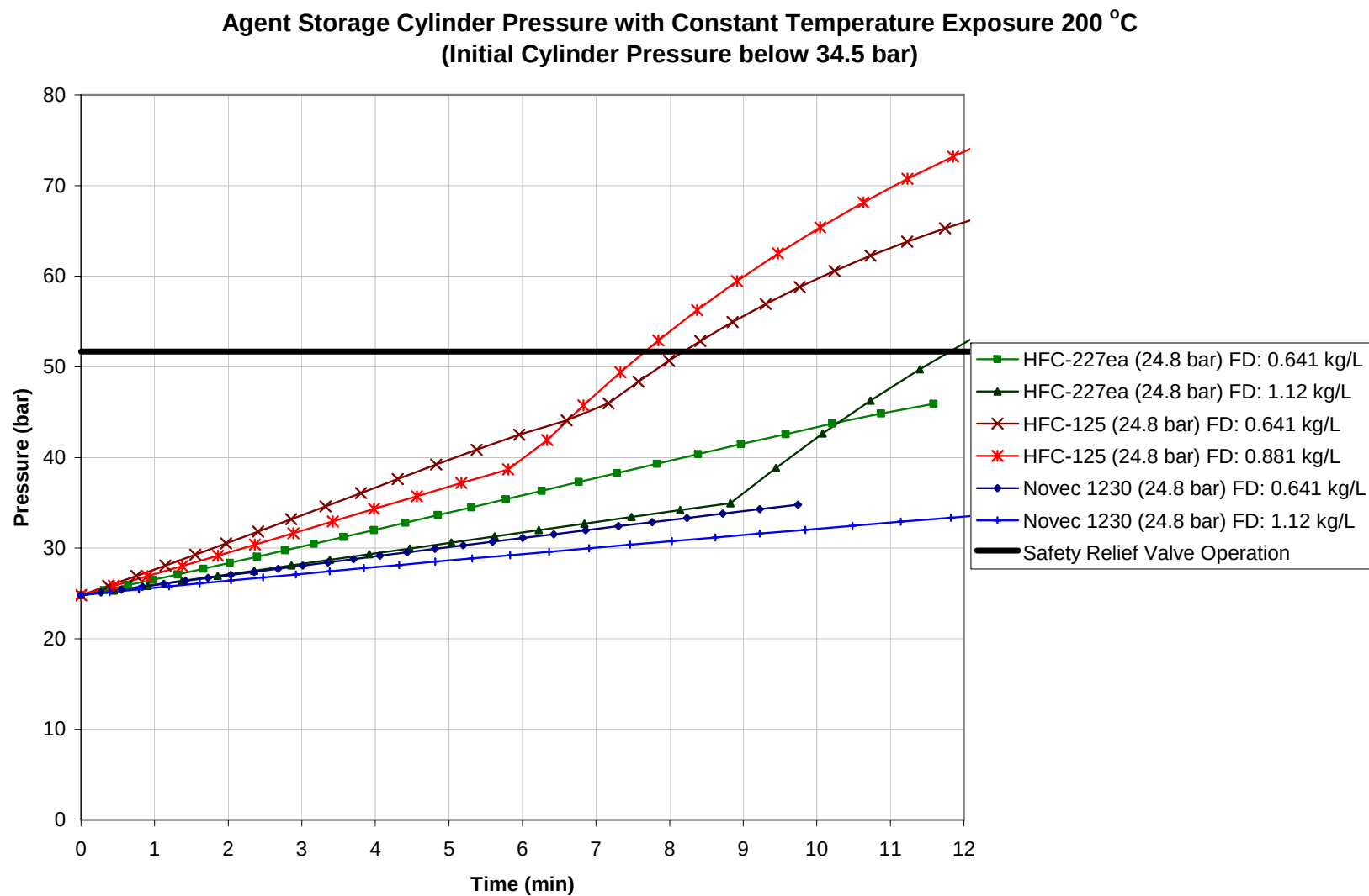
Figure 10. Cylinder Pressure with Constant Temperature Exposure of 200 °C (Low Pressure Cylinders).
