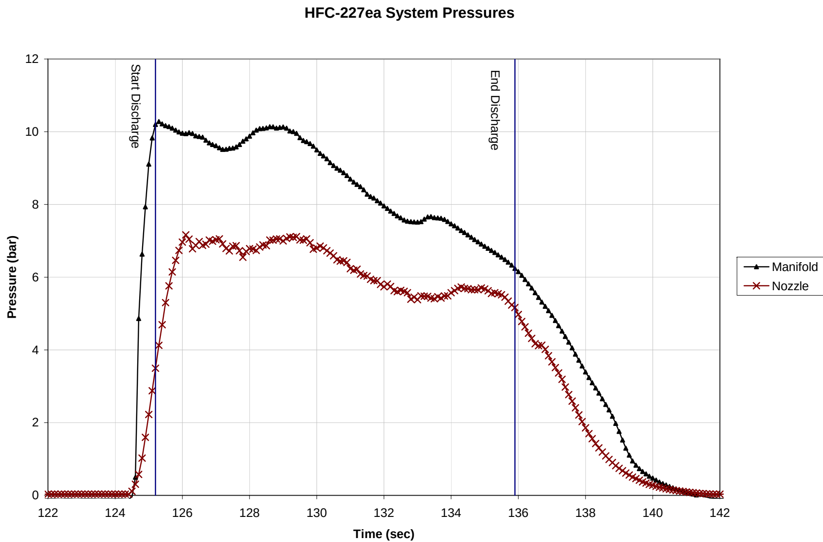
Figure 18. Degraded System Operating Pressure.
