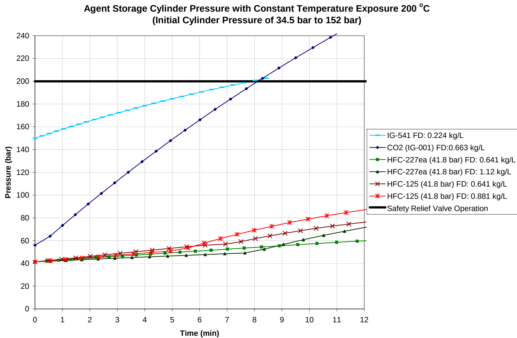
Figure 9. Agent Cylinder Pressure versus Time (High Pressure Cylinders).
