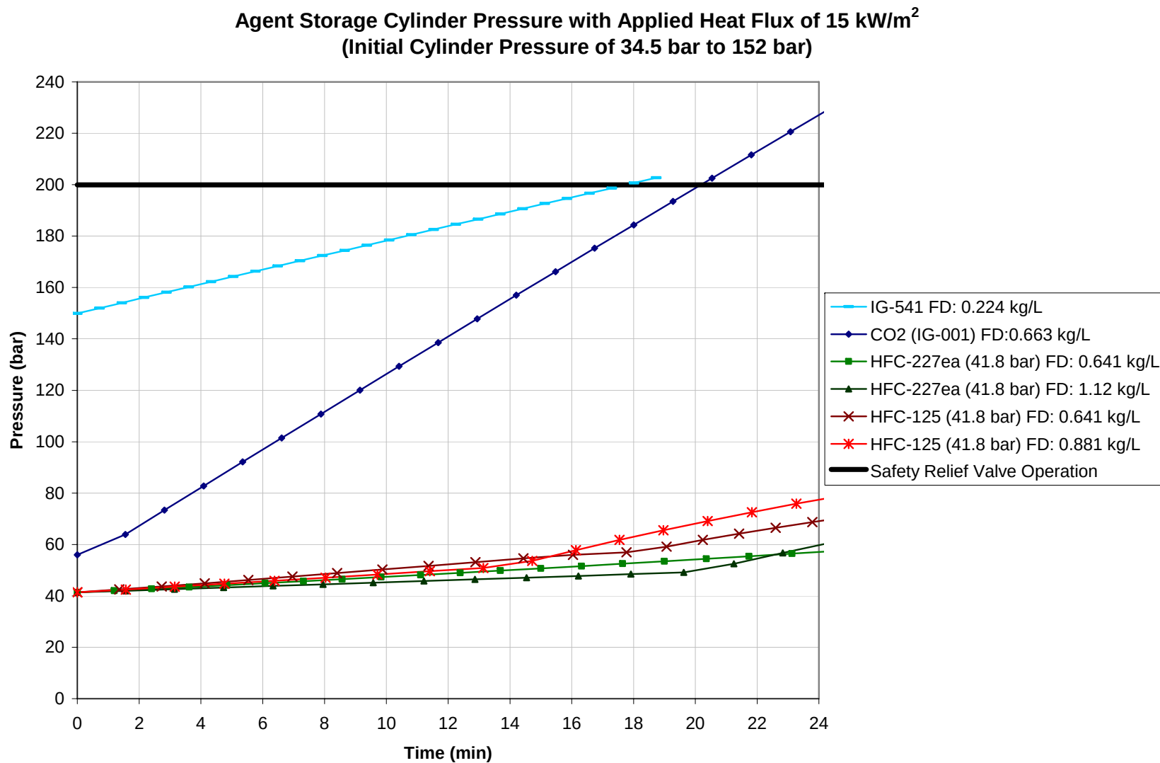
Figure 11. Cylinder Pressure with Constant Temperature Exposure of 200°C (High Pressure Cylinders).
