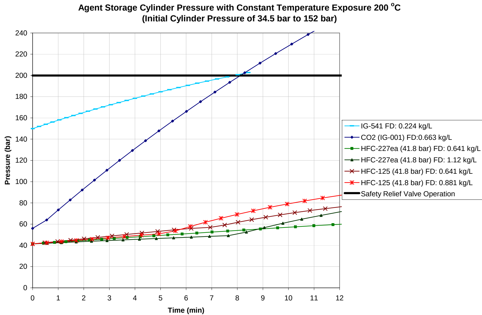
Figure 7. Agent Cylinder Pressure versus Temperature (High Pressure Cylinders).
