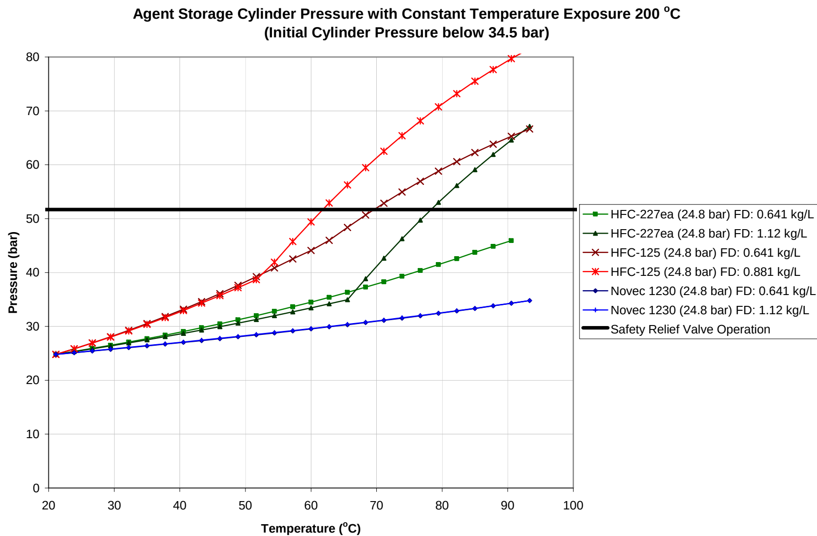
Figure 6. Agent Cylinder Pressure versus Temperature (Low Pressure Cylinders).
