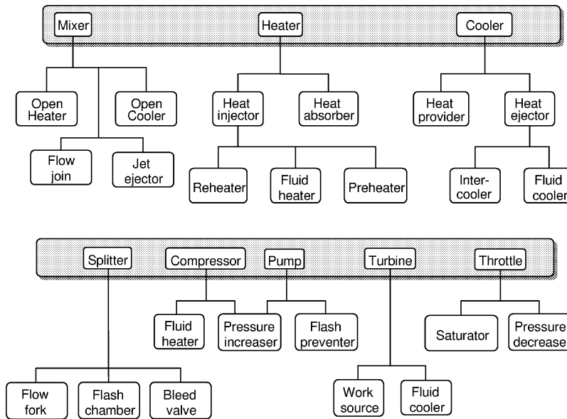
Fig. 6. Role taxonomy.
