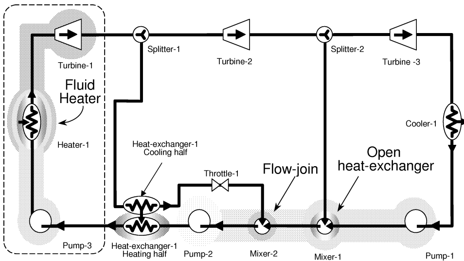
Fig. 8. Adjacency.
