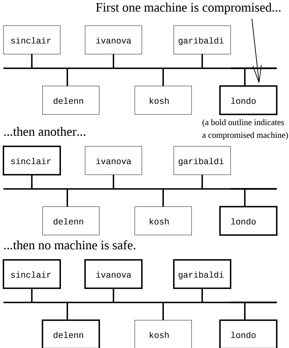
Figure 2: Breaking the circle of trust in a small cluster.
