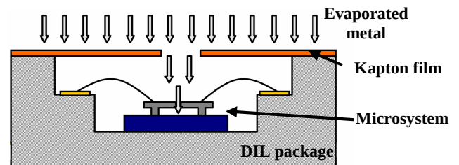
Figure 6 - Drawing of the cross-section of the encapsulated packaged microsystem during metal deposition.
