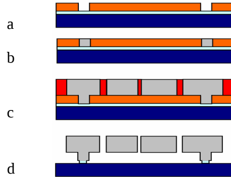
Figure 4 – Process flow.
