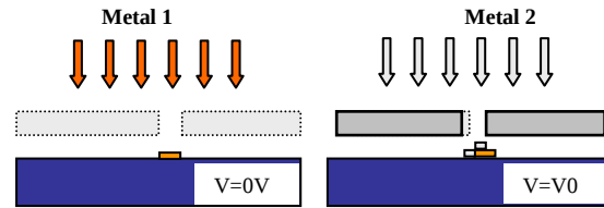
Figure 1 - Concept of the active shutter and shadow mask. a) A first deposition occurs when no voltage is applied. Deposited material reaches the substrate through the opening. b) A second deposition begins while the system is actuated. If the displacement of the opening is less than its width, overlap of the two metallic lines will take place.
