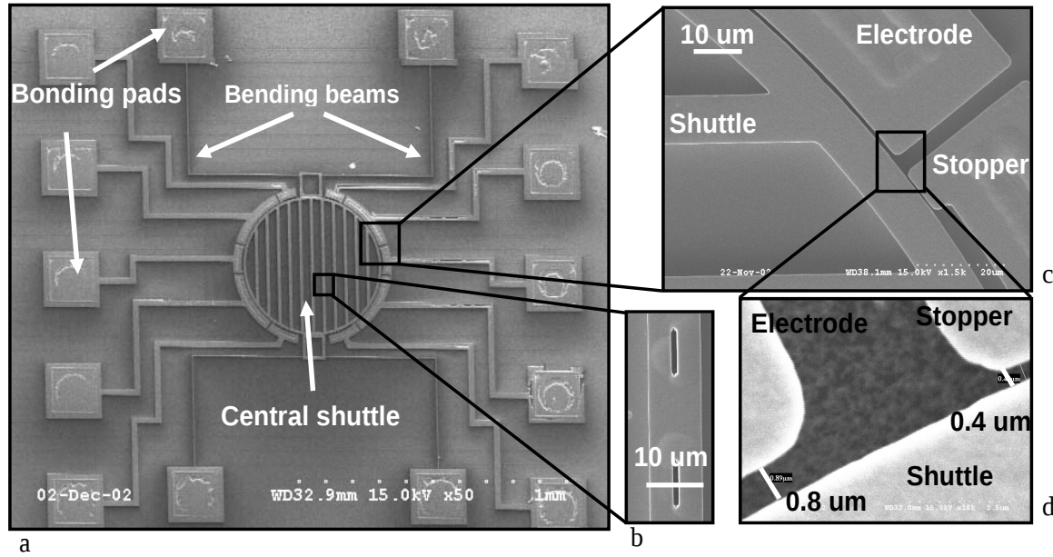
Figure 5 - a) Scanning Electron Micrograph of the overall microactuator. b) Electron micrograph of openings located in the center of the shuttle. c) SEM picture of the side of the shuttle. d) Close-up SEM picture showing the gaps between electrode, stopper, and shuttle.
