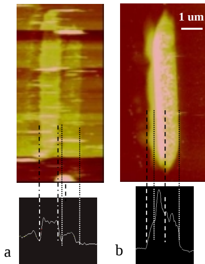
Figure 7 - AFM pictures and cross-section of the deposited metallic lines.
