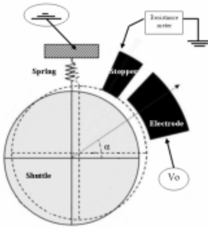
Figure 2 - Schematic of the microactuator design.
