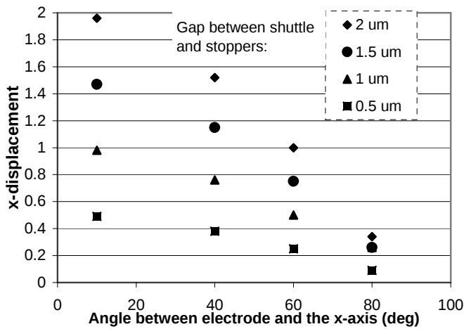
Figure 3 – Calculated indexed displacement (Eqs. 1 and 2) of the shuttle in the x-direction as a function of the gaps between stoppers and shuttle and the position of the attracting electrode.
