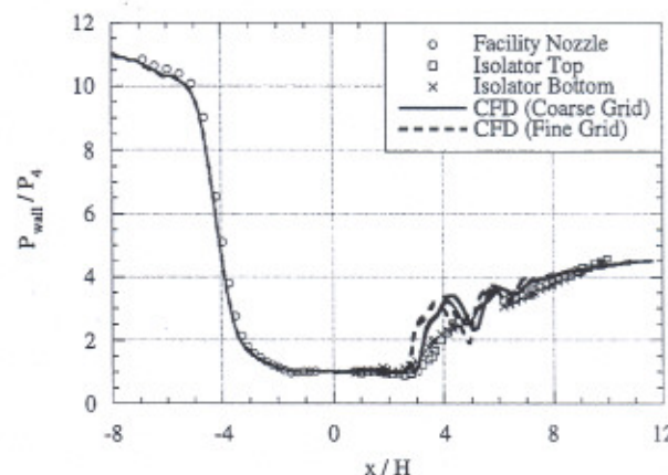
b) Comparison of CFD coarse and fine grid solutions for case 1 ( P_{a1}/P_4 = 4.50 )
