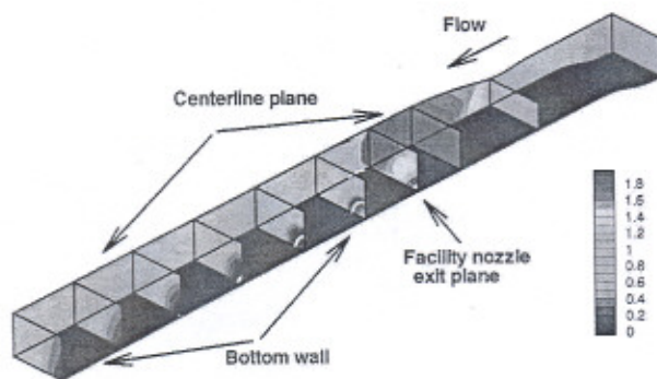
Fig. 8 Calculated Mach number contours from case 1 at P_{01}/P_4 = 3.52 (zero streamwise velocity indicated by a white line).
