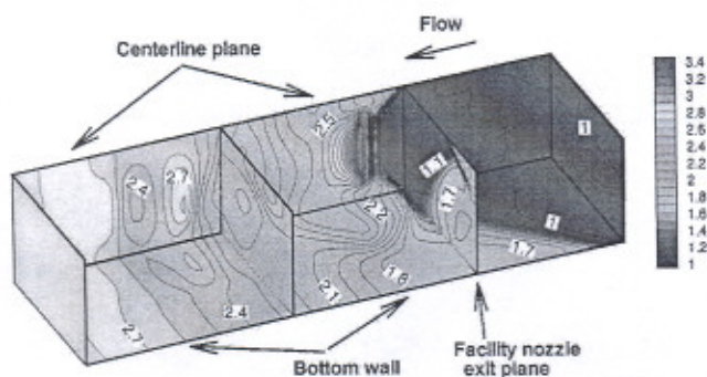
Fig. 9 Calculated normalized static pressure contours from case 1 at P_{01}/P_4 = 3.52 in the vicinity of the shock train.
