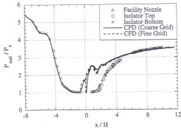
b) Comparison of CFD coarse and fine grid solutions for case 1 ( P_{01}/P_4 = 3.52 )
