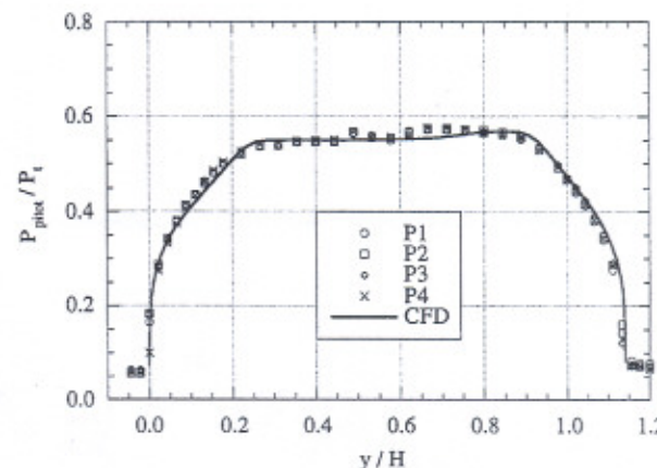
Fig. 13 Normalized isolator exit plane pitot pressure distributions from case 9 at P_{a1}/P_4 = 0.94 .
