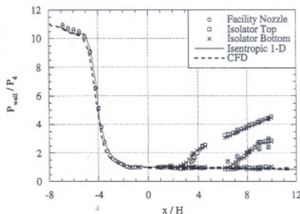
a) Case 9 with three levels of backpressure
