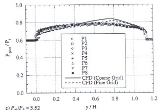
Fig. 10 Normalized isolator exit plane pitot pressure distributions from case 1.
