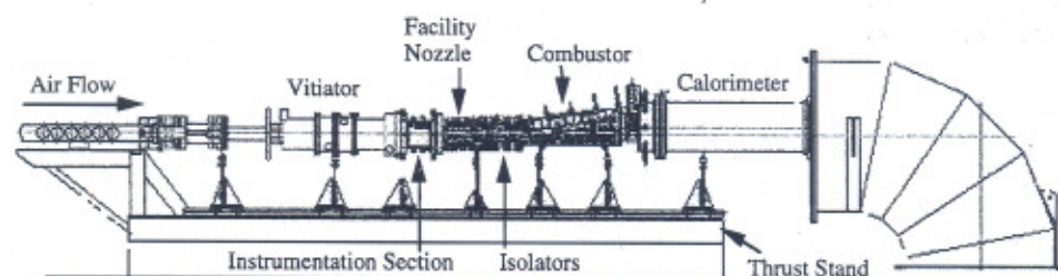
Fig. 2 Facility schematic.
