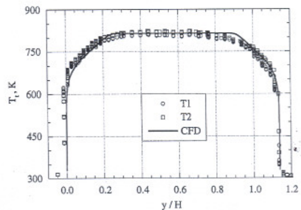
Fig. 11 Normalized isolator exit plane total temperature distributions from case 1 at P_{01}/P_4 = 0.97 .
