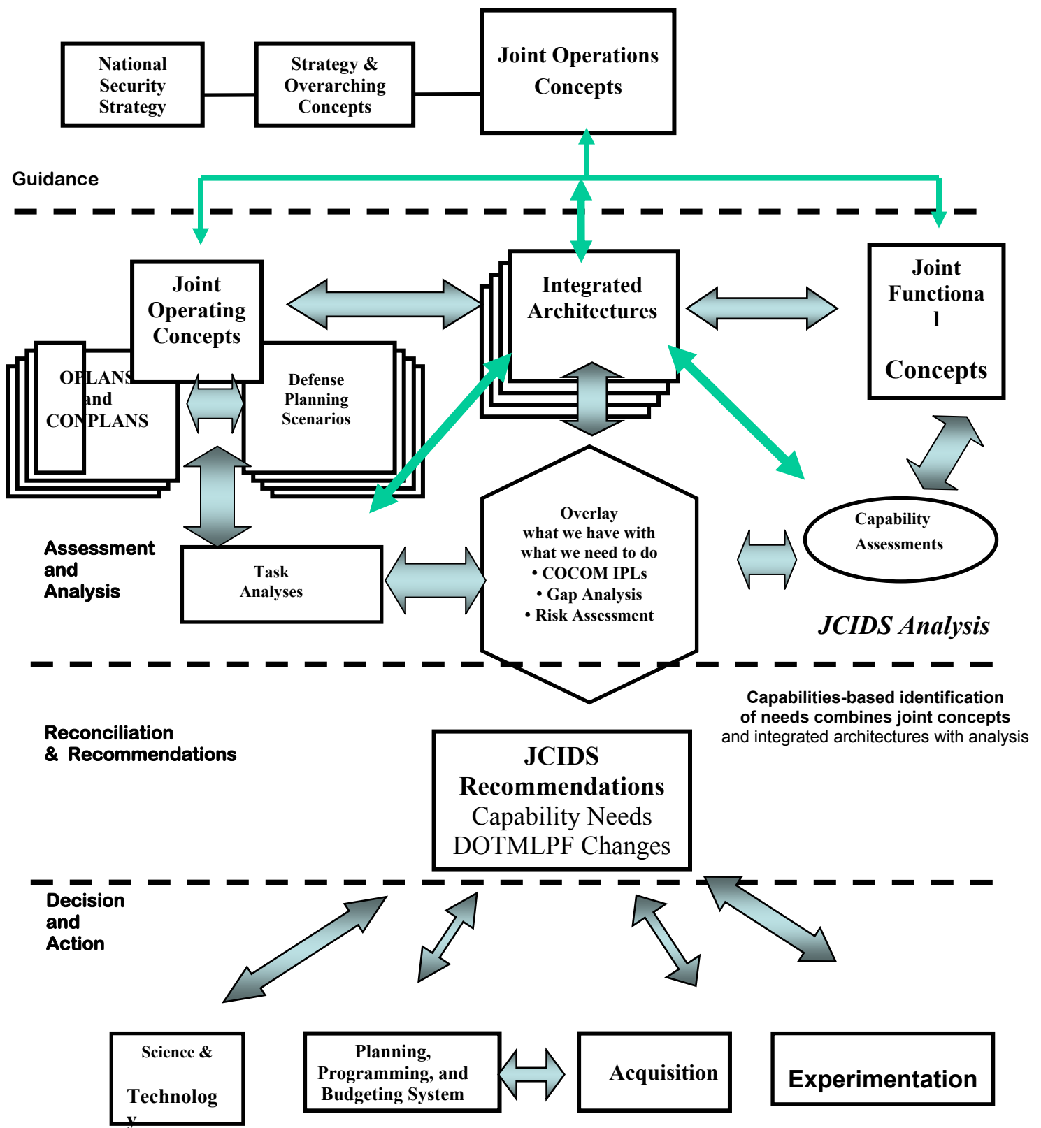
Figure 3 JCIDS Process
