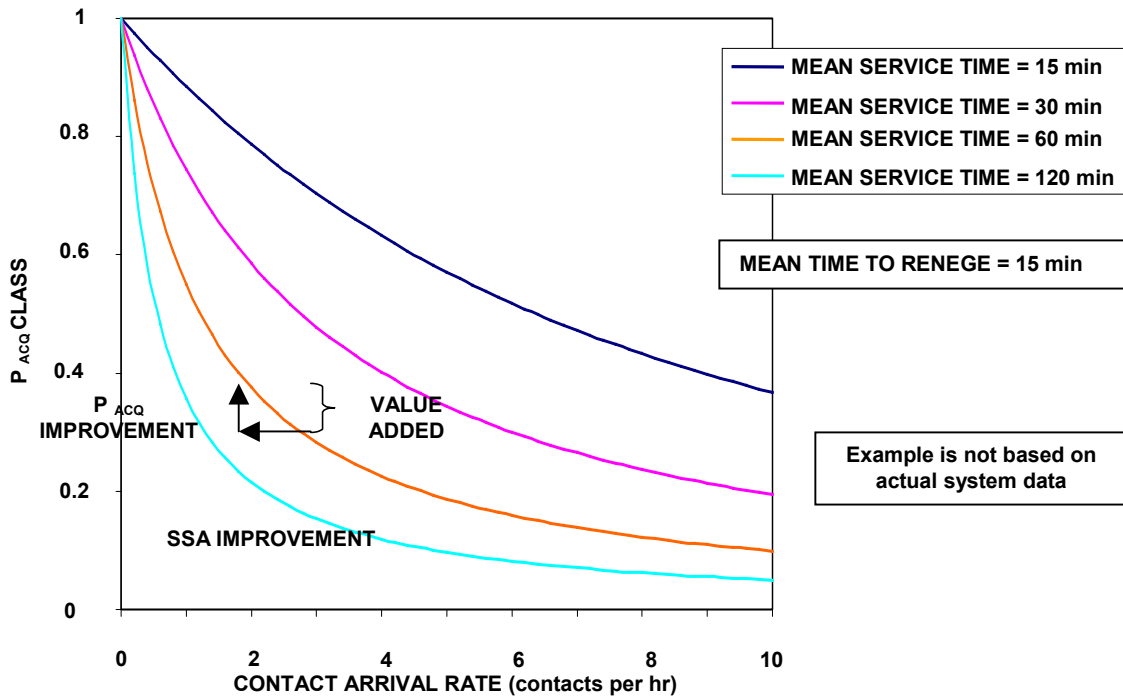
Figure 4: Effect of Improved SSA on Probability of Acquisition, P_{ACQ}
