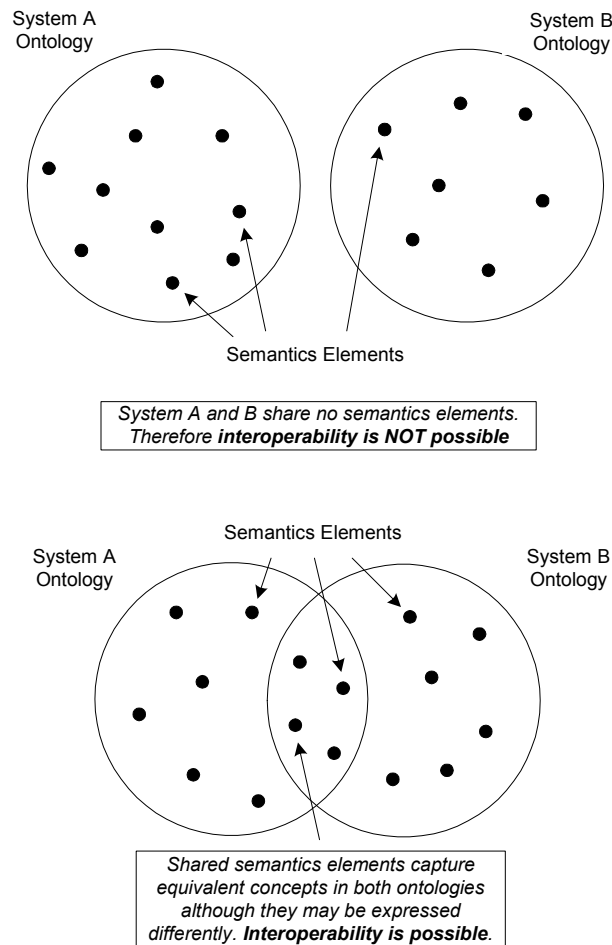
Figure 1: Semantic-level Interoperability
