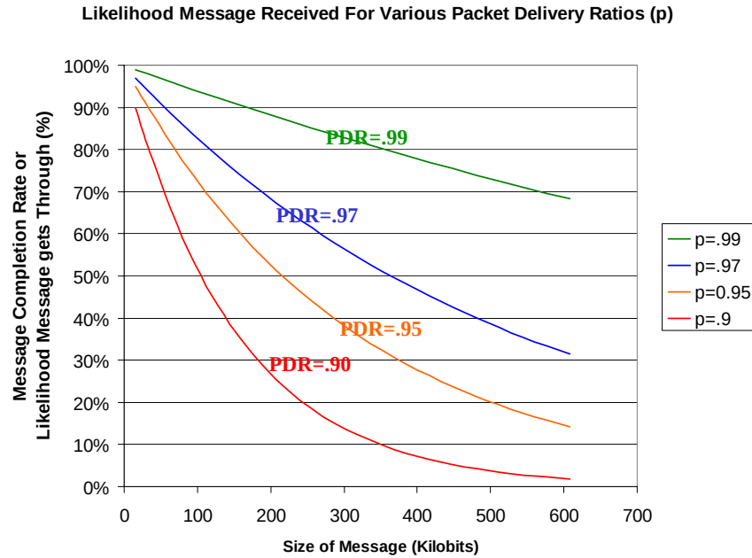
Figure 20: Packet Delivery Ratio and MCR
