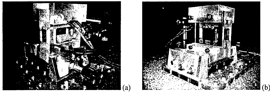
Figure 15. JHU/APL miniature thrust stand. (a) Front. (b) Back.
