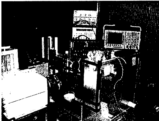
Figure 10. Experimental setup for micro-PIV studies of the SparkJet device.
