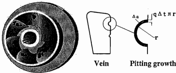
Figure 5: Schematic corrosion/erosion damage to the vanes (left) and schematic pitting growth model (right)
