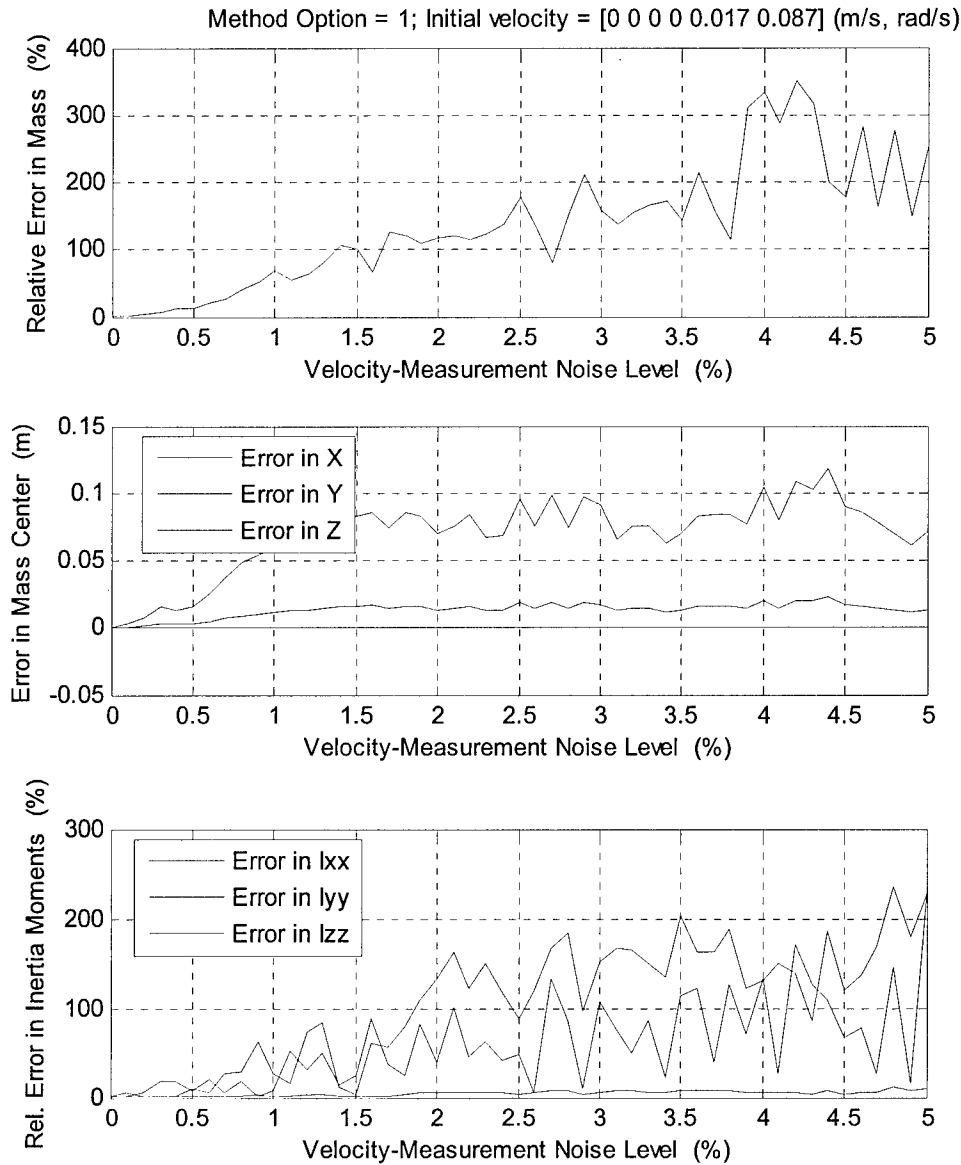
Fig. 23 Identification errors when different noises are added to the angular velocity measurement (Note: the error in the position of the mass center is represented by the absolute error because the mass center is located at the origin and thus the relative error is undefined)
