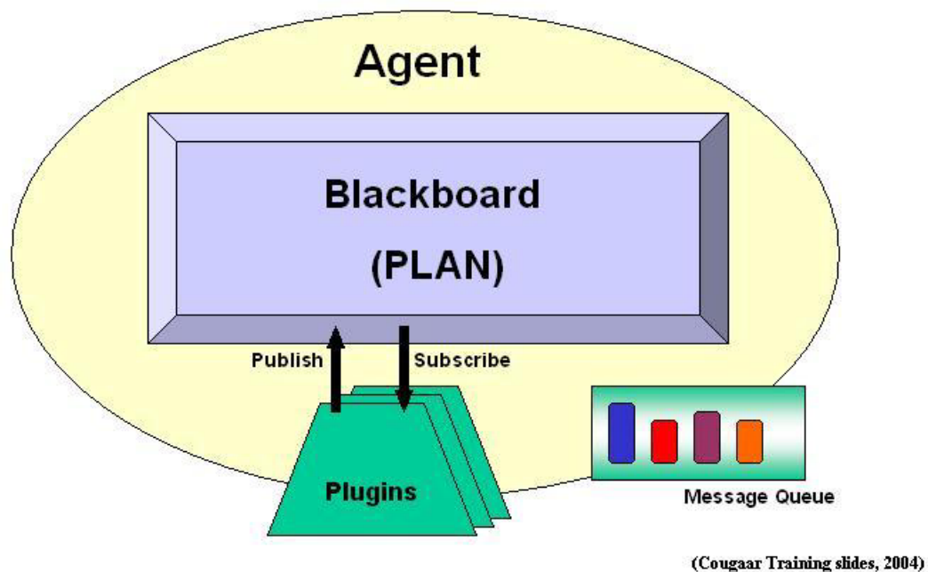
Figure 1. Cougaar agent anatomy
