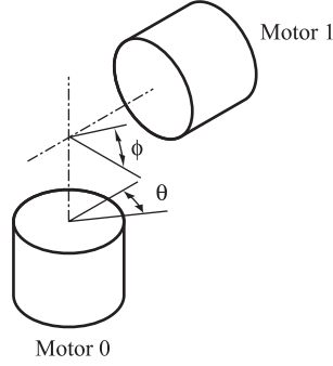
Figure 2.7: Arrangement of Motors
