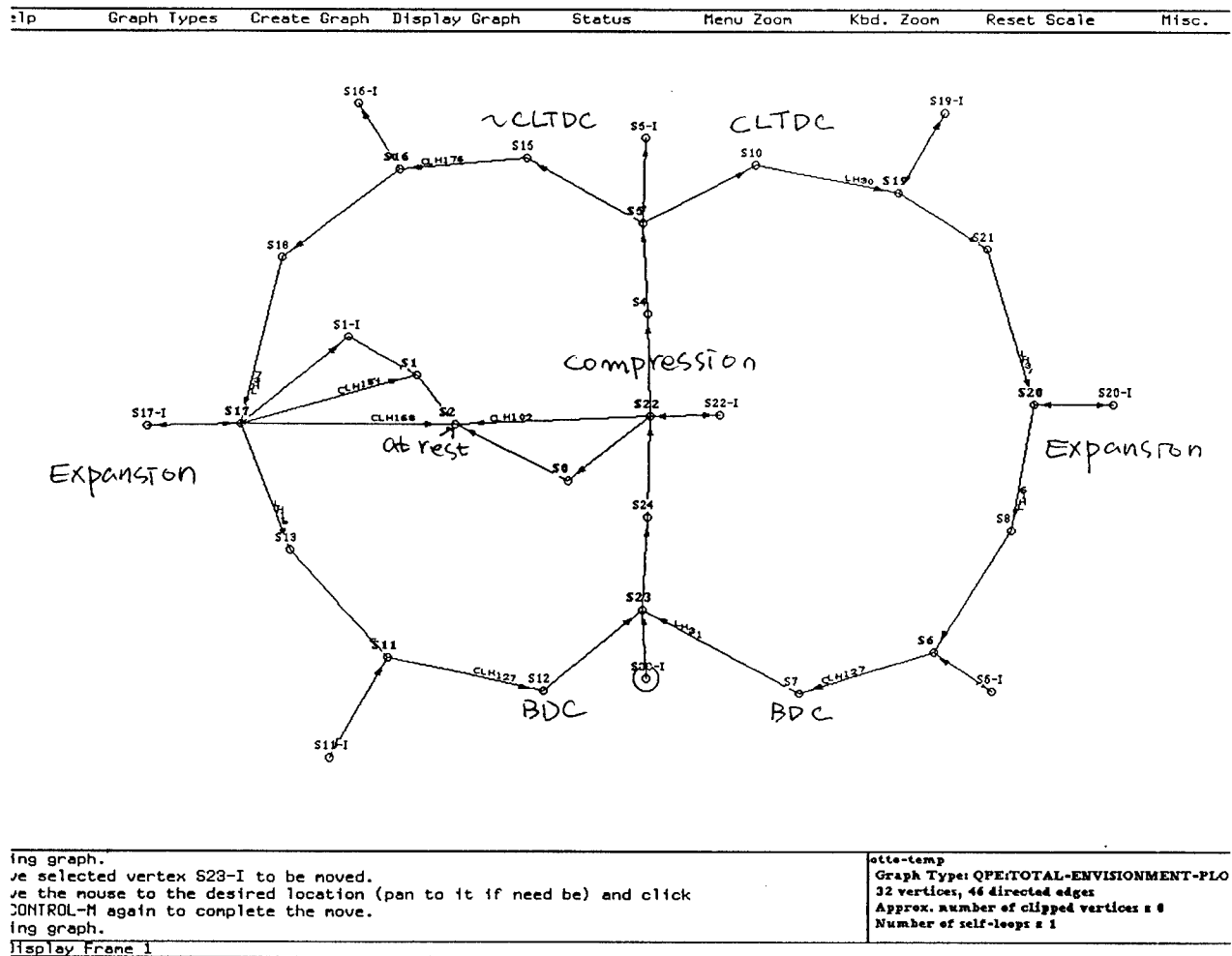
Figure 7.11: Envisionment of a piston-cylinder system with event CLTDC.
