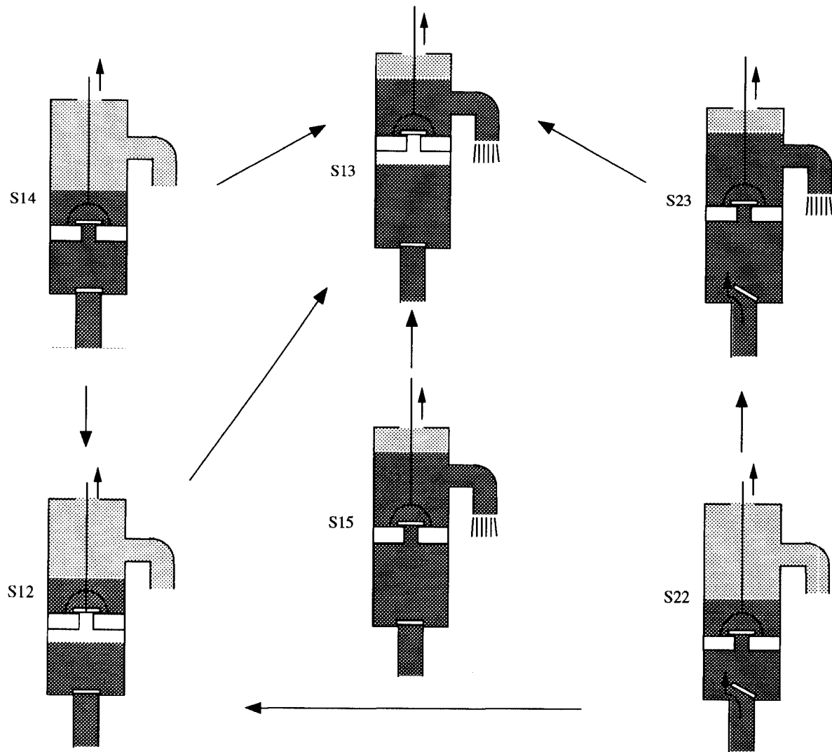
Figure 8.13: Part of the envisionment corresponding to step 3.
