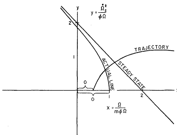
Figure A3 - Relation between actual relay pull-in and drop-out and phase plane trajectory
