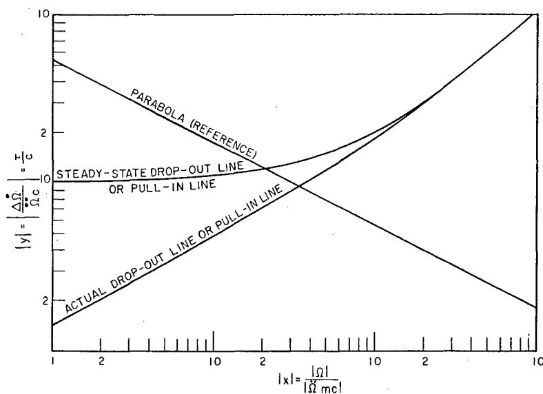
Figure A4 - Transient correction for relay drop-out or pull-in line when an acceleration exists
