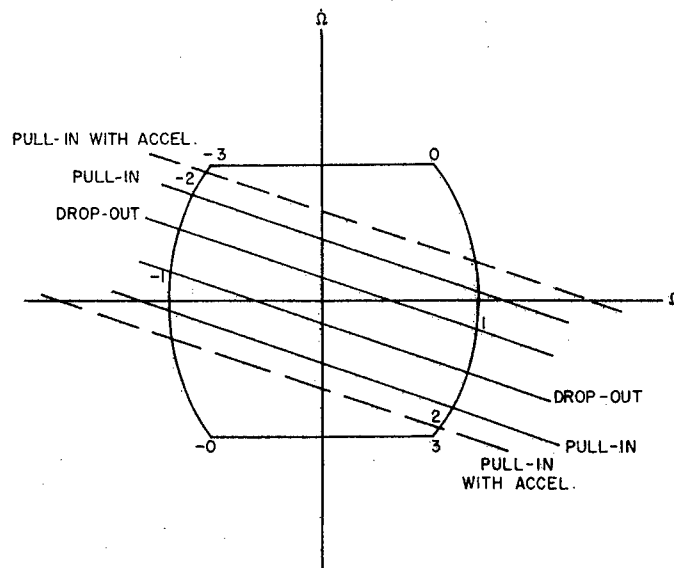
Figure 6 - Over-compensated system
