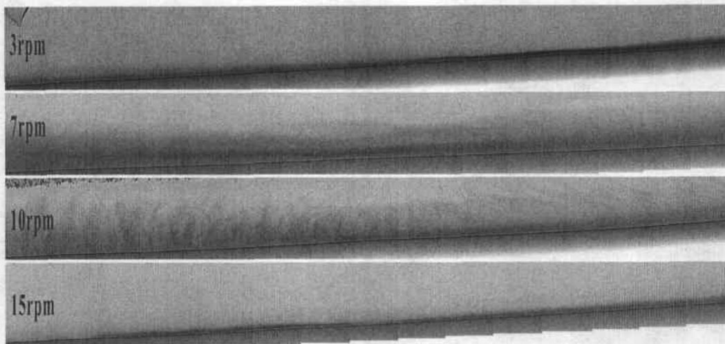
Figure 27: Test 2, the variation of field lines in the magnetic fluid with 10wt% \text{Fe}_3\text{O}_4 under fixed magnetic field but different flow speeds.
