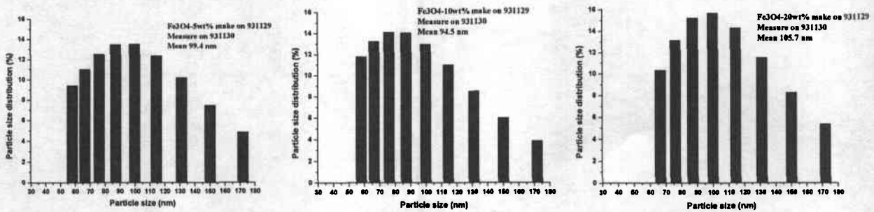
Figure 5. The particle size distributions of \text{Fe}_3\text{O}_4 with different concentrations; from left are 5wt%, 10 wt% and 20 wt%, respectively.
